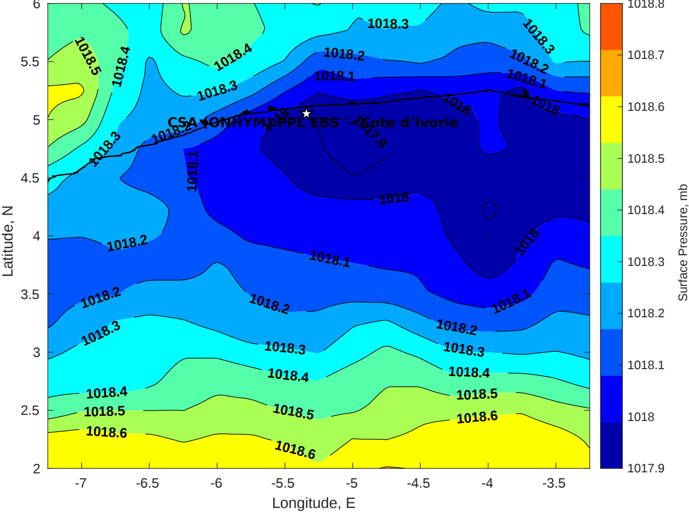
Surface Pressure (mb) for CSA (ONHYM) PPL EBS - Cote d'Ivoire at 14-Jul-2025 00:00:00
