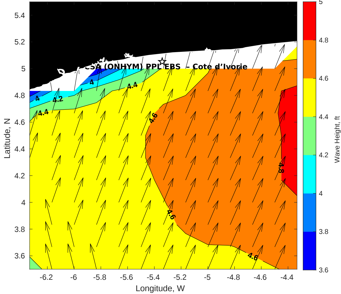
Wave Height (ft) for CSA (ONHYM) PPL EBS - Cote d'Ivoire at 12-Jul-2025 09:00:00
