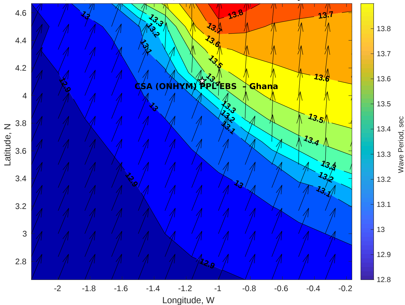
Wave Period (sec) for CSA (ONHYM) PPL EBS - Ghana at 12-Jul-2025 09:00:00
