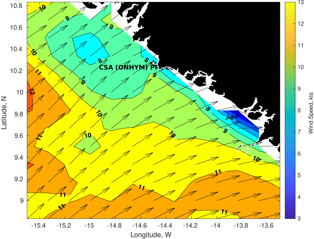
Winds (kts) for CSA (ONHYM) PPL EBS - Guinea at 12-Jul-2025 09:00:00
