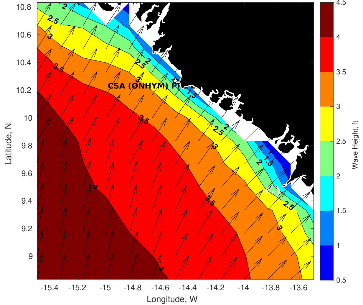
Wave Height (ft) for CSA (ONHYM) PPL EBS - Guinea at 12-Jul-2025 09:00:00
