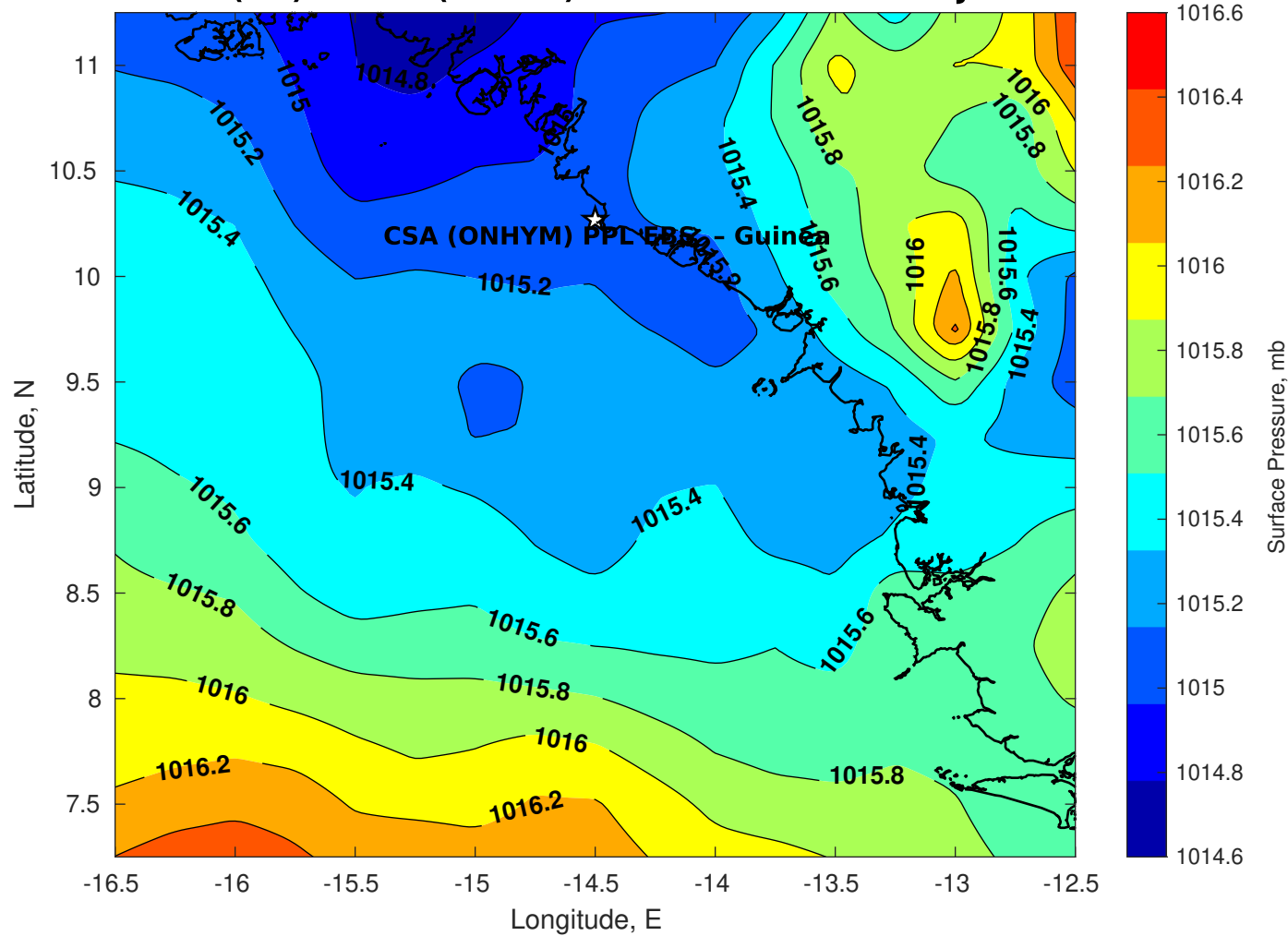
Surface Pressure (mb) for CSA (ONHYM) PPL EBS - Guinea at 13-Jul-2025 00:00:00
