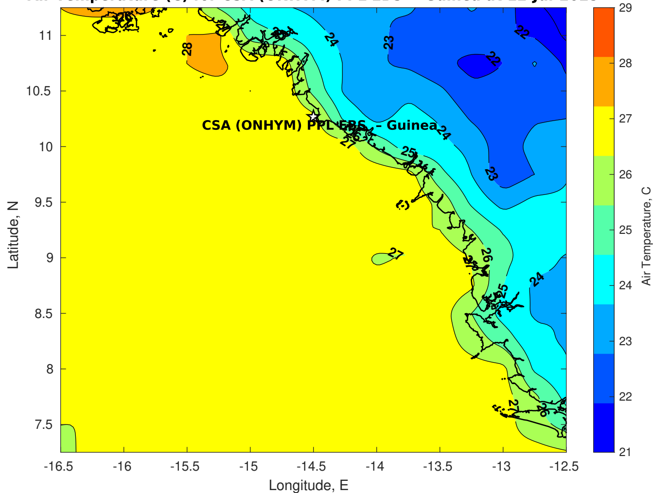
Air Temperature (C) for CSA (ONHYM) PPL EBS - Guinea at 12-Jul-2025
