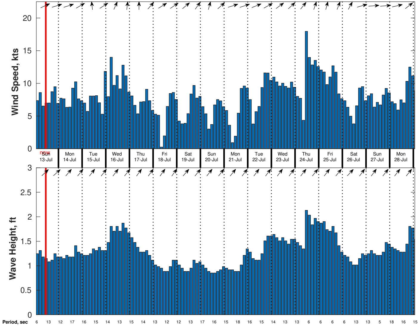
Wind & Wave Forecast for CSA (ONHYM) PPL EBS - Guinea from 12-Jul-2025 01:00:00 to 28-Jul-2025 01:00:00
