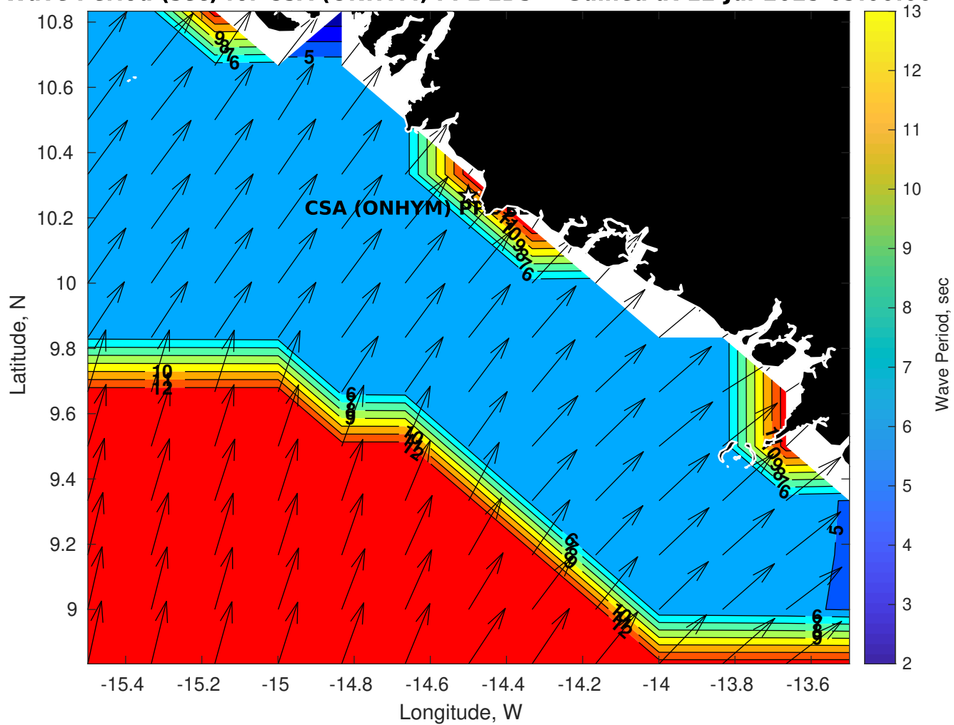
Wave Period (sec) for CSA (ONHYM) PPL EBS - Guinea at 12-Jul-2025 09:00:00
