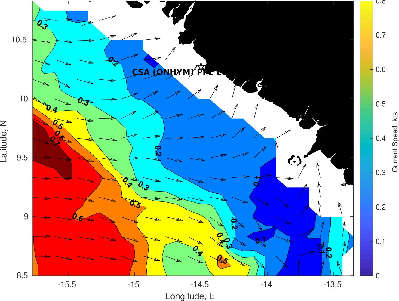
Surface Currents for CSA (ONHYM) PPL EBS - Guinea at 11-Jul-2025 00:00:00
