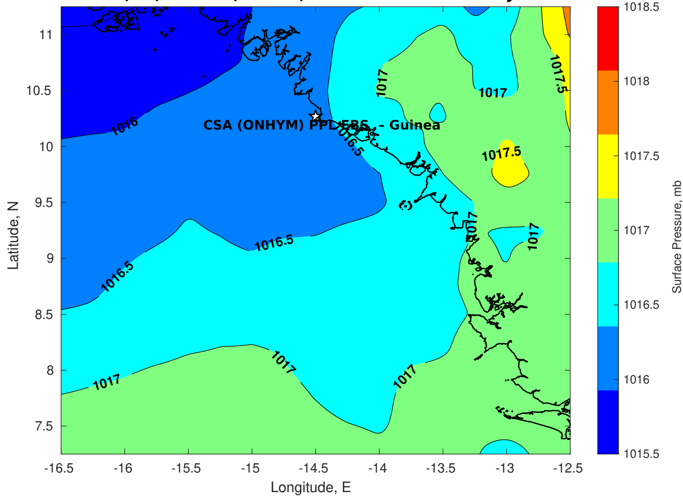
Surface Pressure (mb) for CSA (ONHYM) PPL EBS - Guinea at 14-Jul-2025 00:00:00
