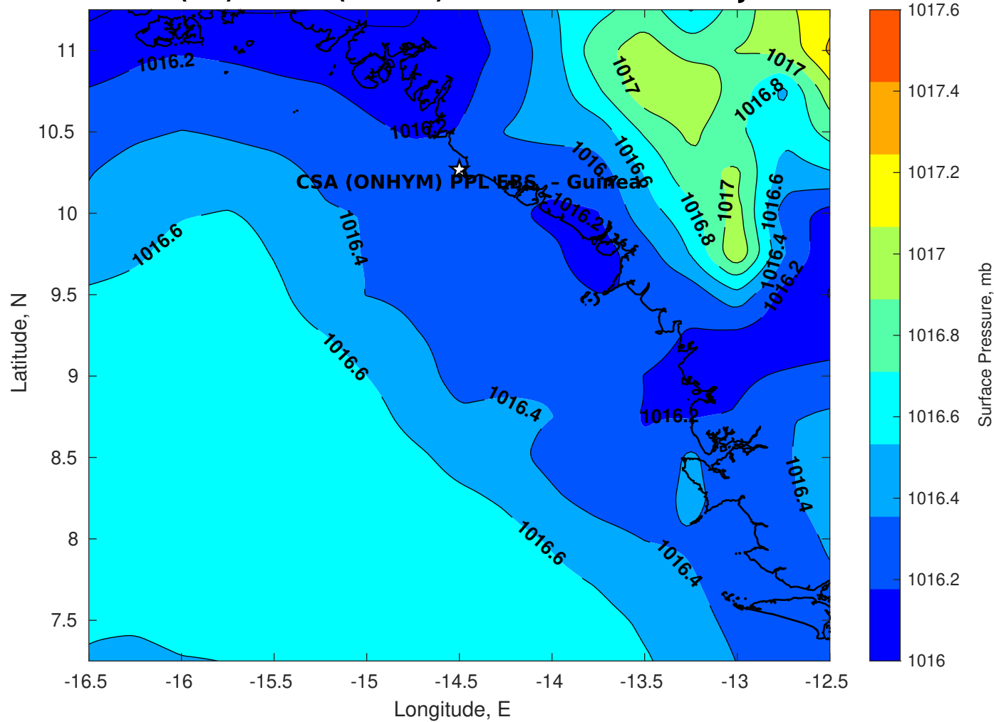
Surface Pressure (mb) for CSA (ONHYM) PPL EBS - Guinea at 12-Jul-2025 00:00:00
