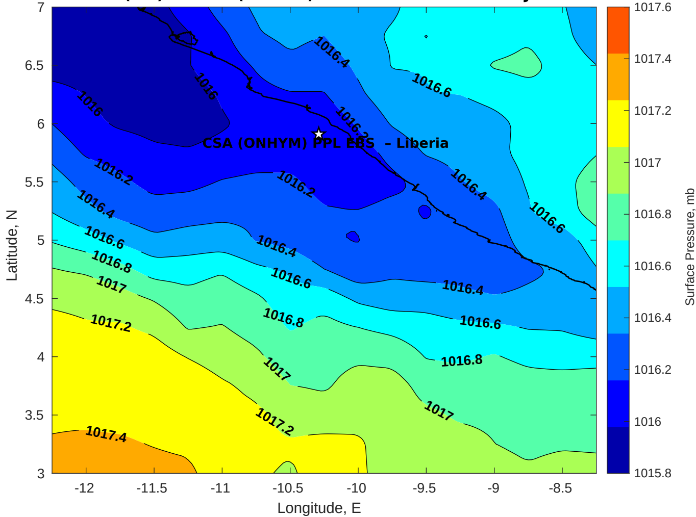
Surface Pressure (mb) for CSA (ONHYM) PPL EBS - Liberia at 13-Jul-2025 00:00:00
