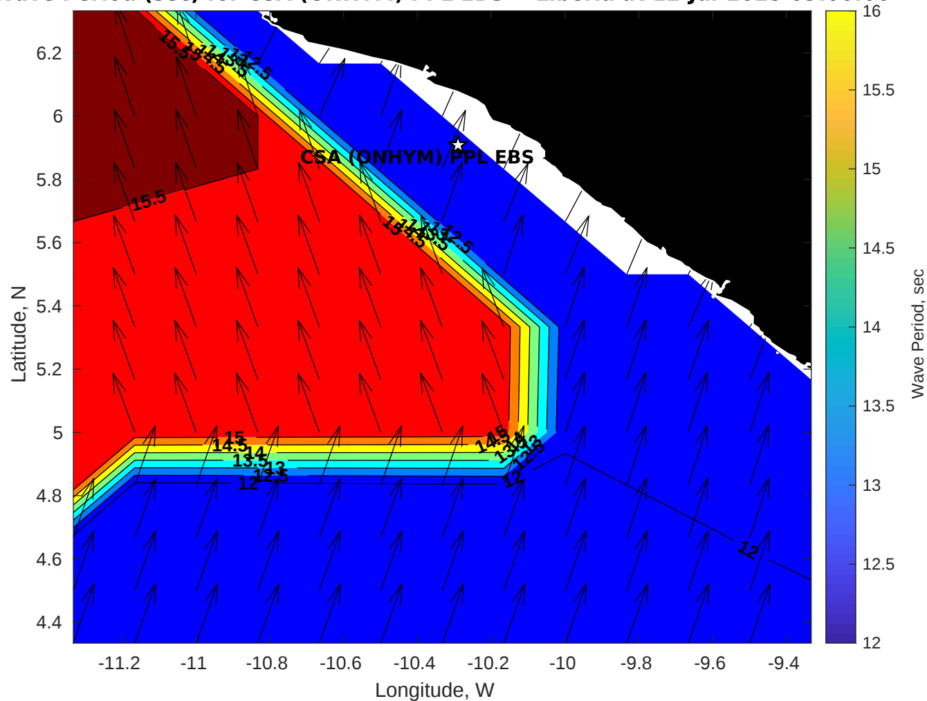
Wave Period (sec) for CSA (ONHYM) PPL EBS - Liberia at 12-Jul-2025 09:00:00
