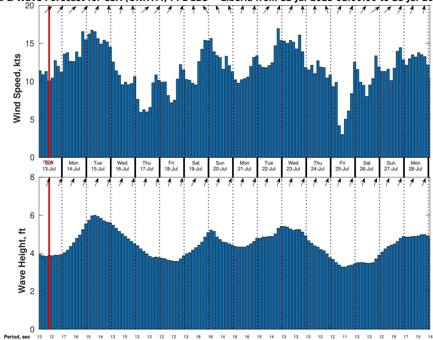
Wind & Wave Forecast for CSA (ONHYM) PPL EBS - Liberia from 12-Jul-2025 01:00:00 to 28-Jul-2025 01:00:00
