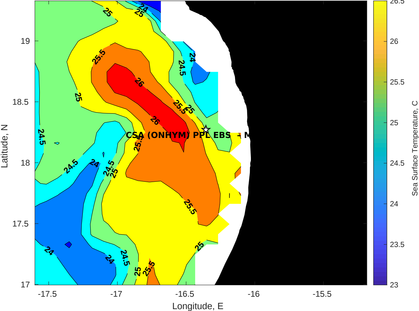
SST for CSA (ONHYM) PPL EBS - Mauritania at 11-Jul-2025 00:00:00
