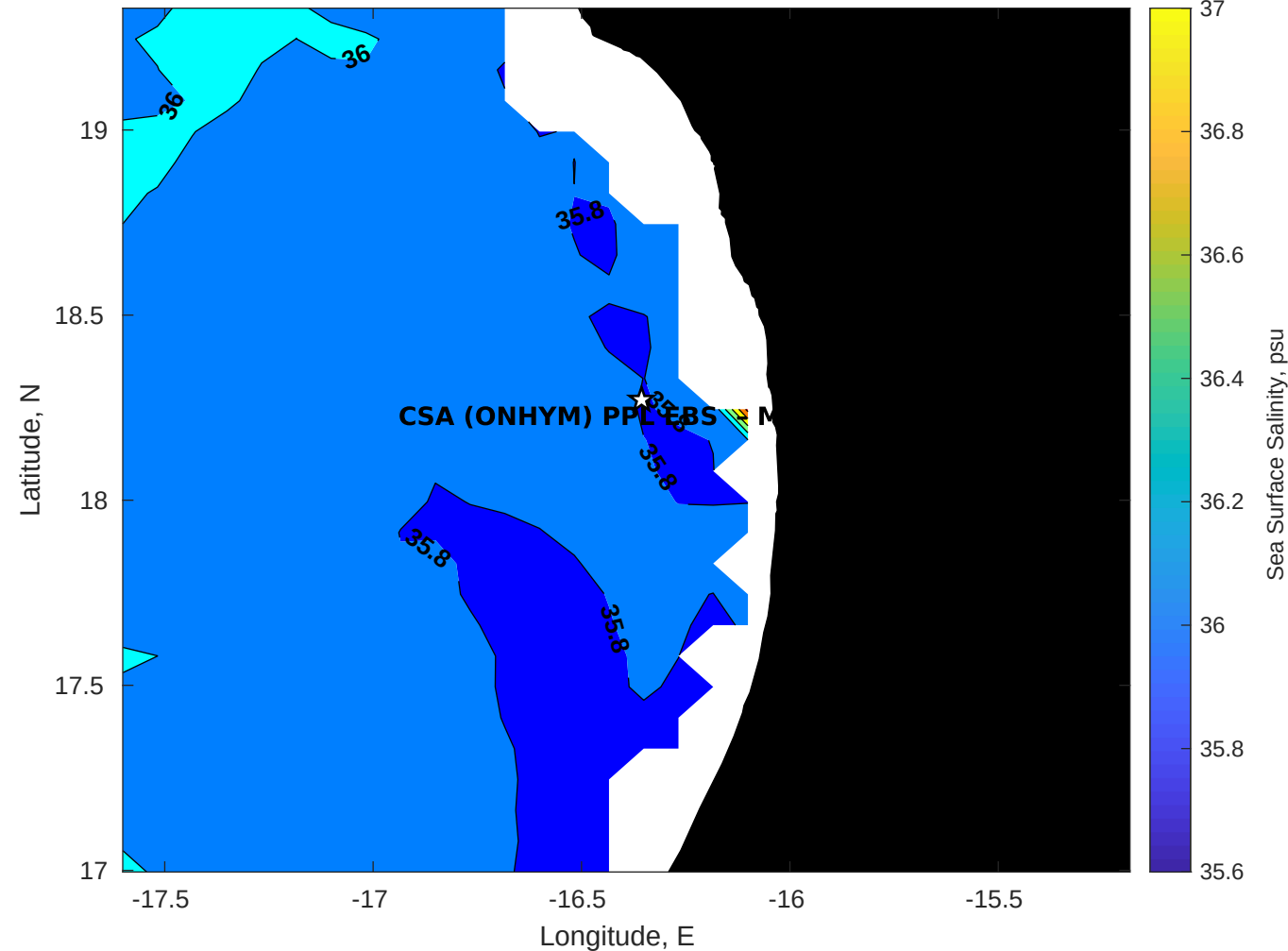
Surface Salinity for CSA (ONHYM) PPL EBS - Mauritania at 11-Jul-2025 00:00:00
