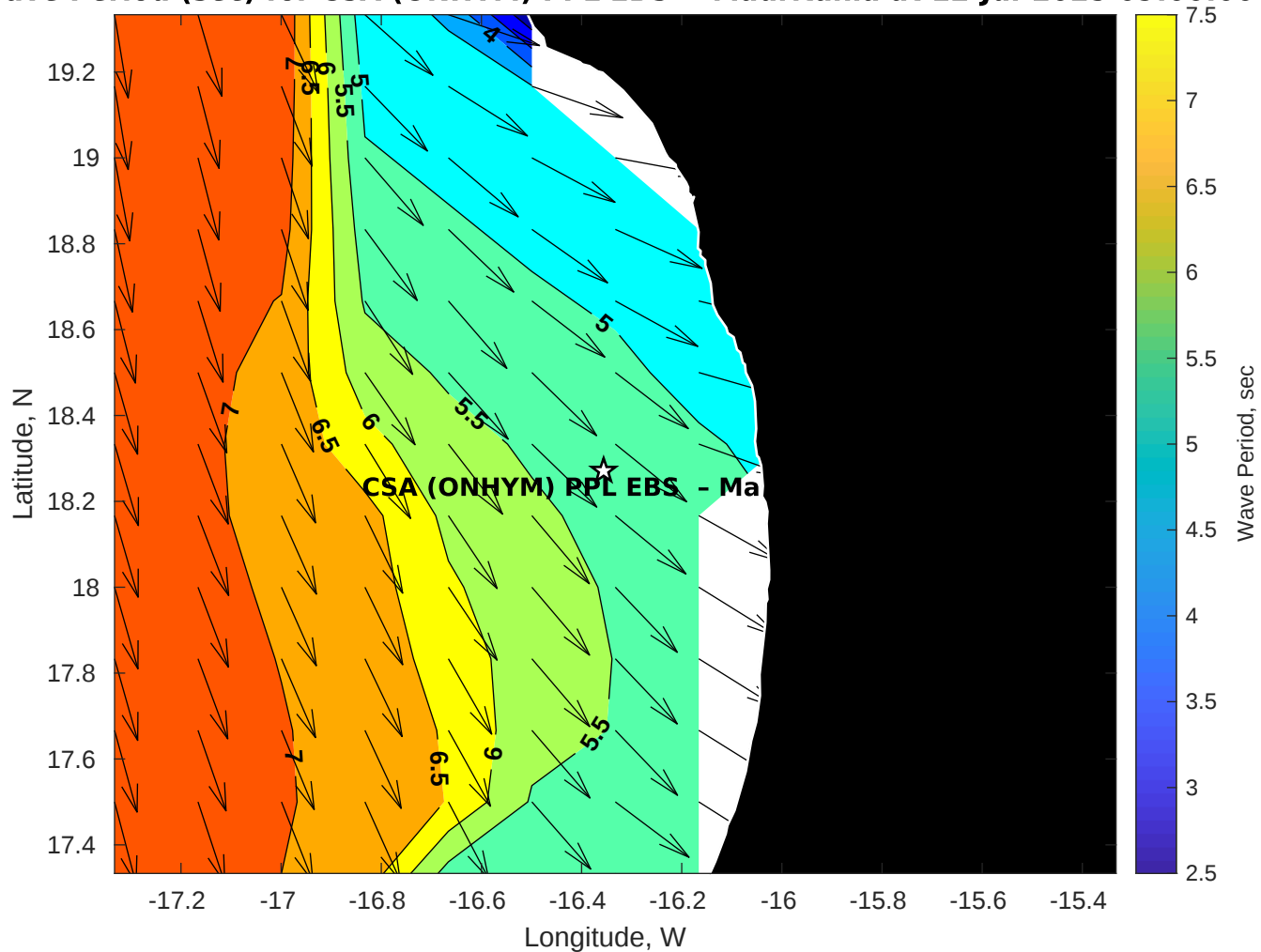
Wave Period (sec) for CSA (ONHYM) PPL EBS - Mauritania at 12-Jul-2025 09:00:00
