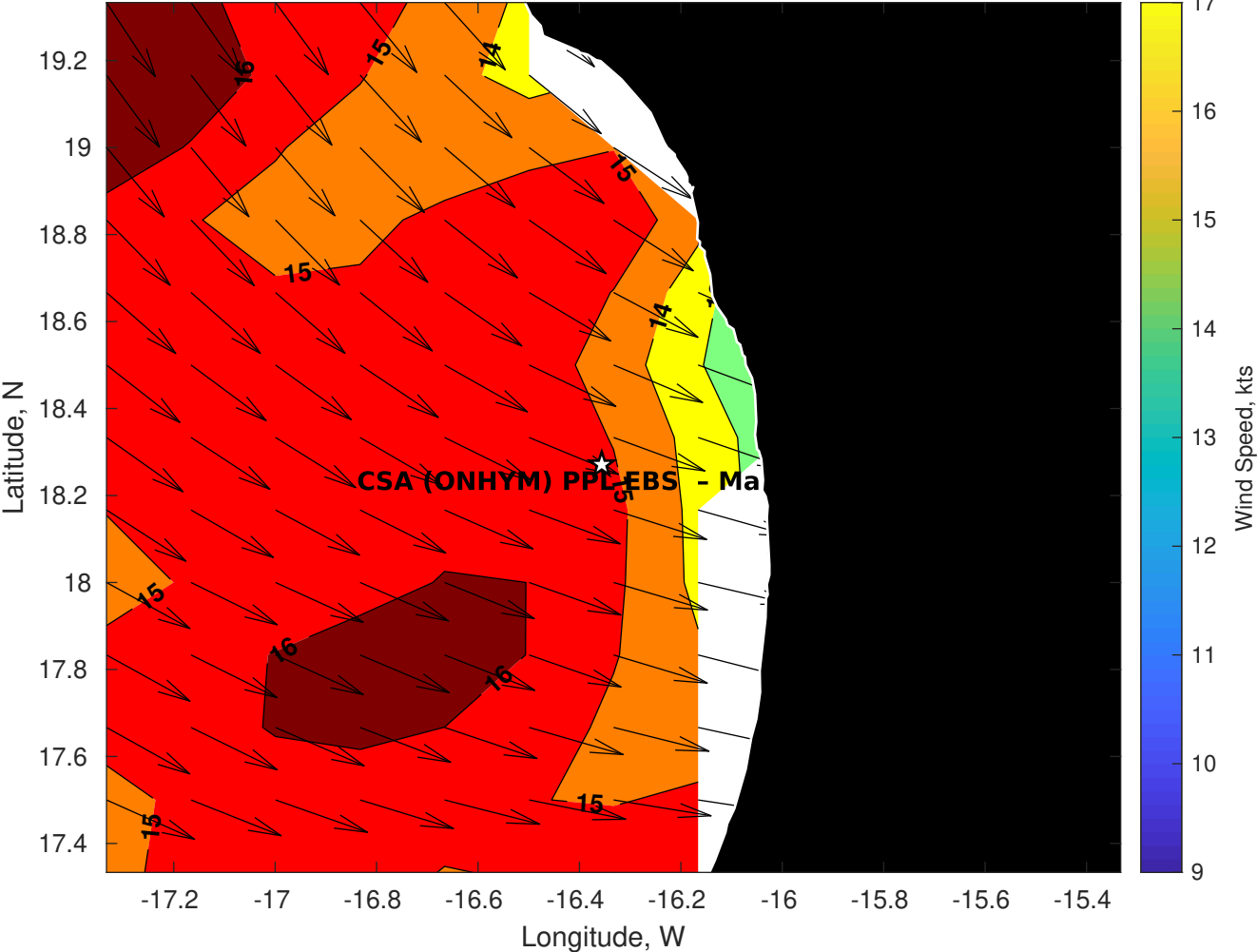
Winds (kts) for CSA (ONHYM) PPL EBS - Mauritania at 12-Jul-2025 09:00:00
