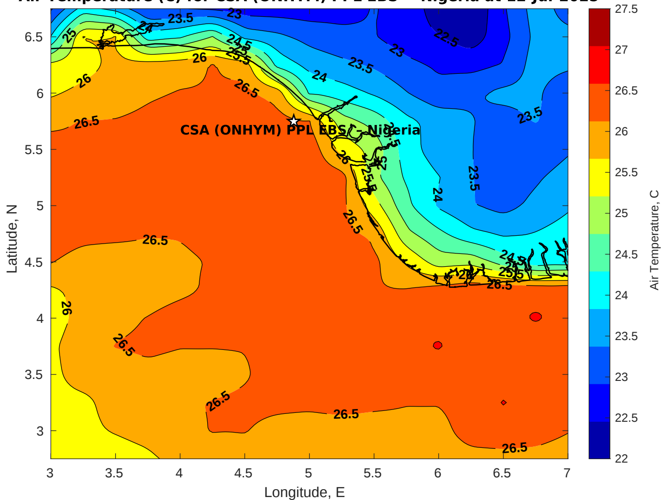
Air Temperature (C) for CSA (ONHYM) PPL EBS - Nigeria at 12-Jul-2025
