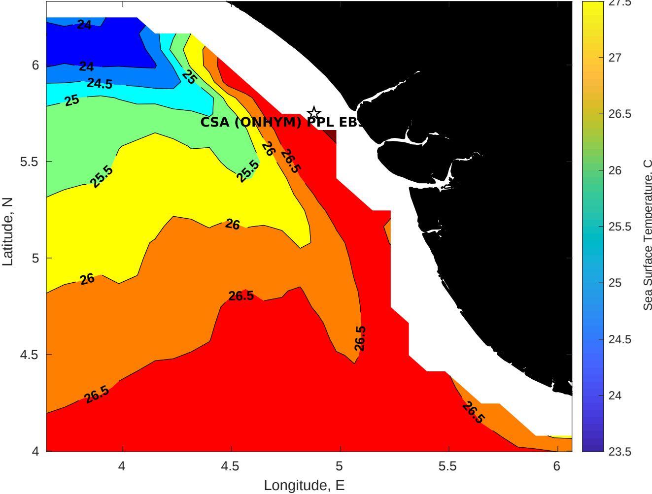
SST for CSA (ONHYM) PPL EBS - Nigeria at 11-Jul-2025 00:00:00
