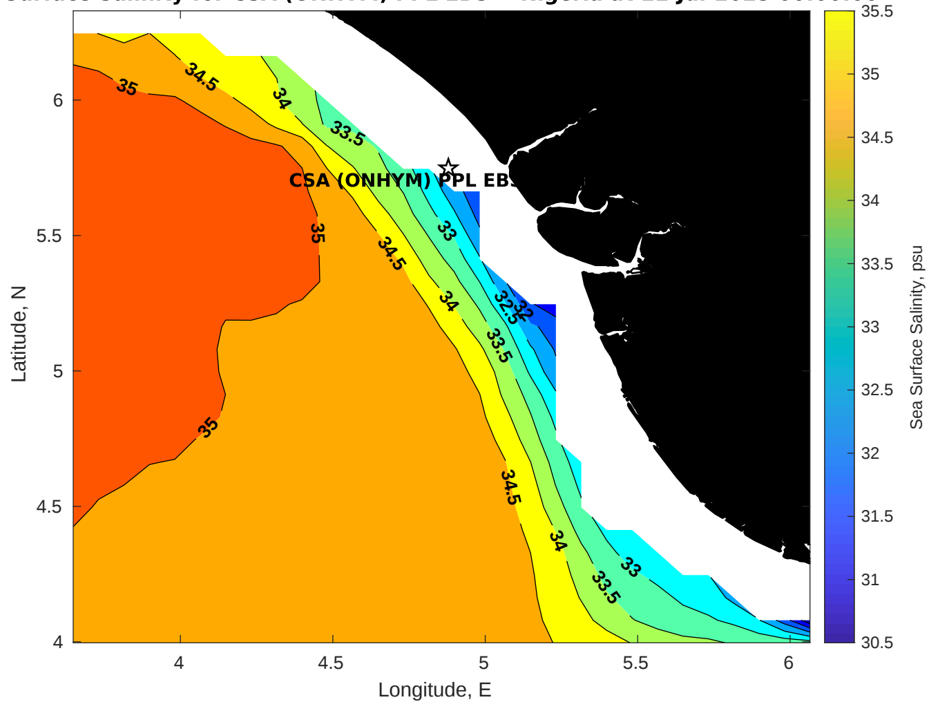
Surface Salinity for CSA (ONHYM) PPL EBS - Nigeria at 11-Jul-2025 00:00:00
