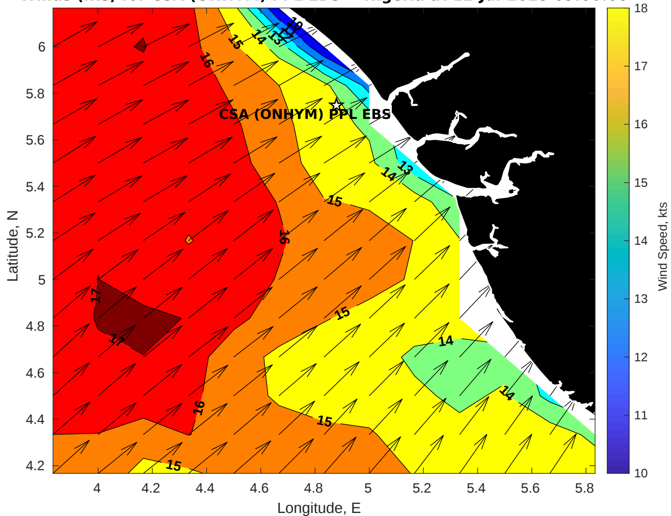
Winds (kts) for CSA (ONHYM) PPL EBS - Nigeria at 12-Jul-2025 09:00:00
