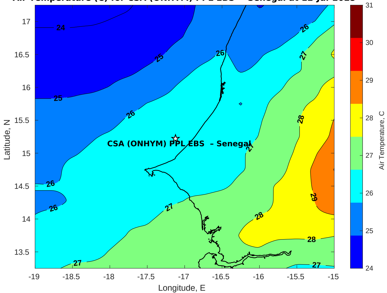
Air Temperature (C) for CSA (ONHYM) PPL EBS - Senegal at 12-Jul-2025
