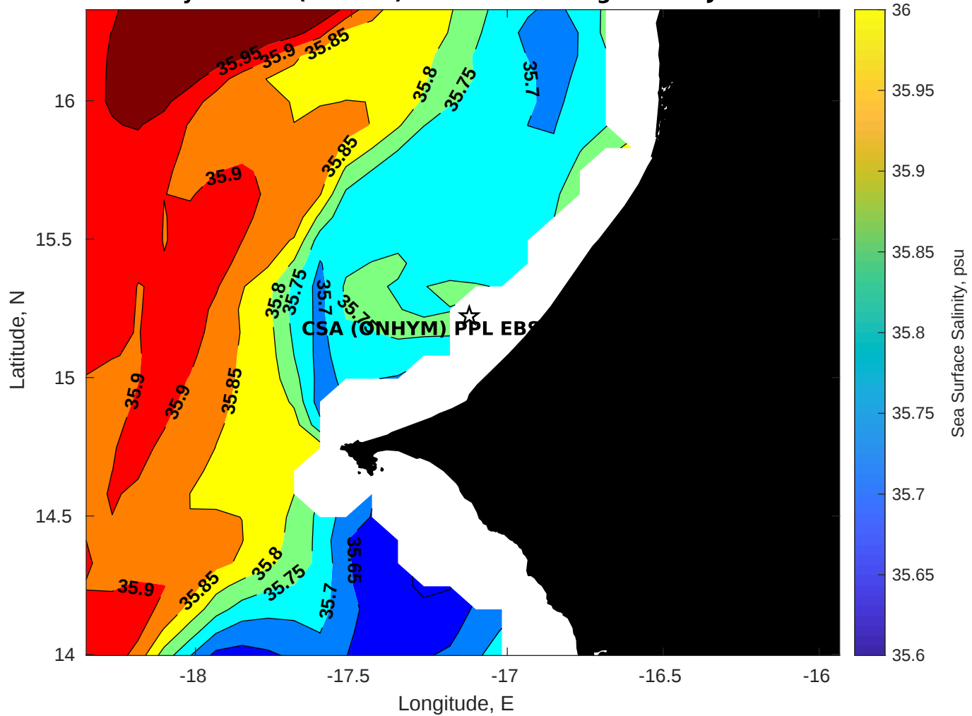
Surface Salinity for CSA (ONHYM) PPL EBS - Senegal at 11-Jul-2025 00:00:00
