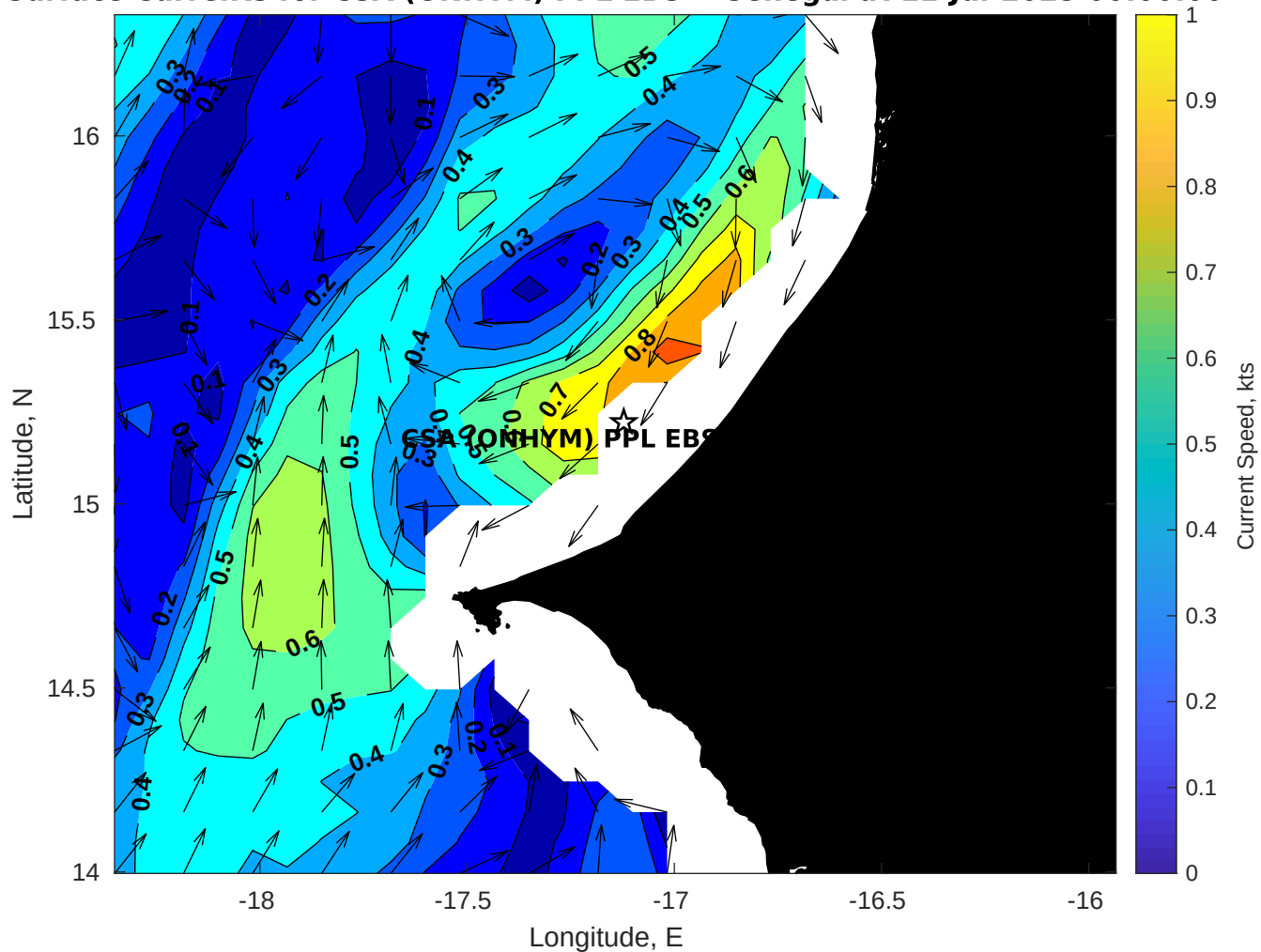
Surface Currents for CSA (ONHYM) PPL EBS - Senegal at 11-Jul-2025 00:00:00
