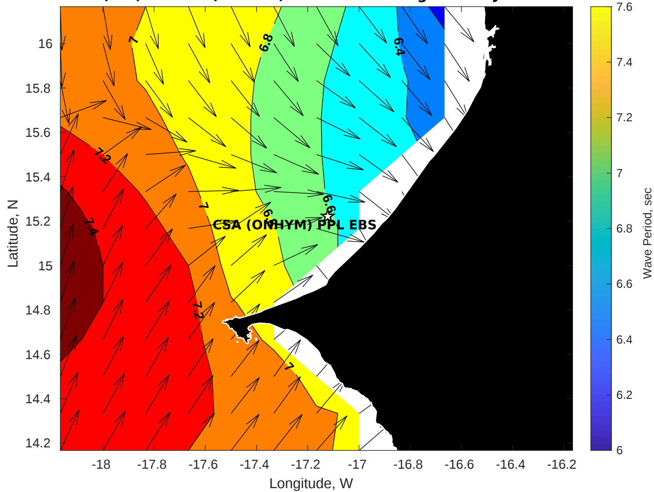
Wave Period (sec) for CSA (ONHYM) PPL EBS - Senegal at 12-Jul-2025 09:00:00
