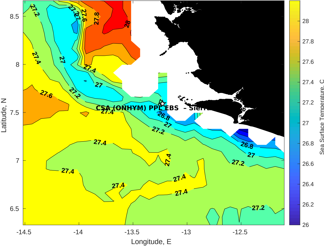
SST for CSA (ONHYM) PPL EBS - Sierra Leone at 11-Jul-2025 00:00:00
