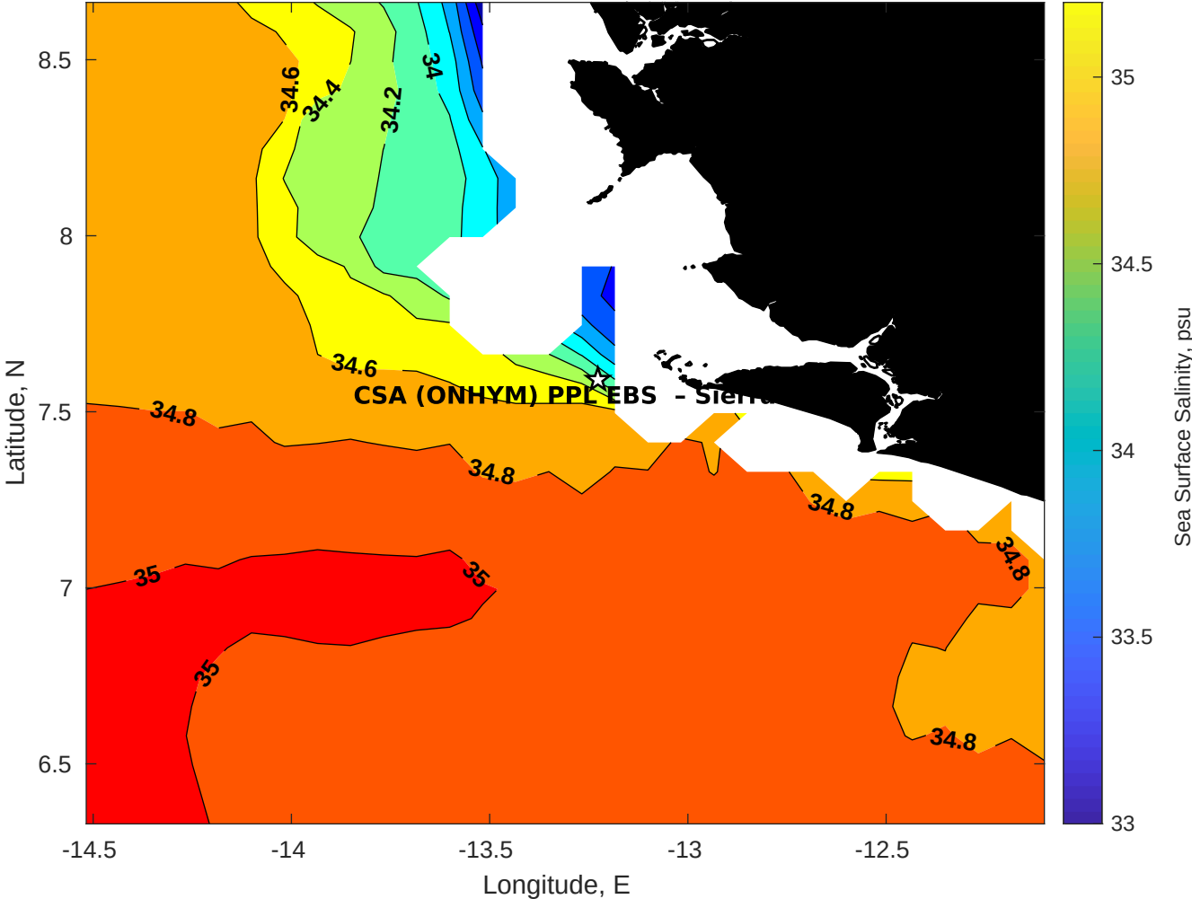
Surface Salinity for CSA (ONHYM) PPL EBS - Sierra Leone at 11-Jul-2025 00:00:00
