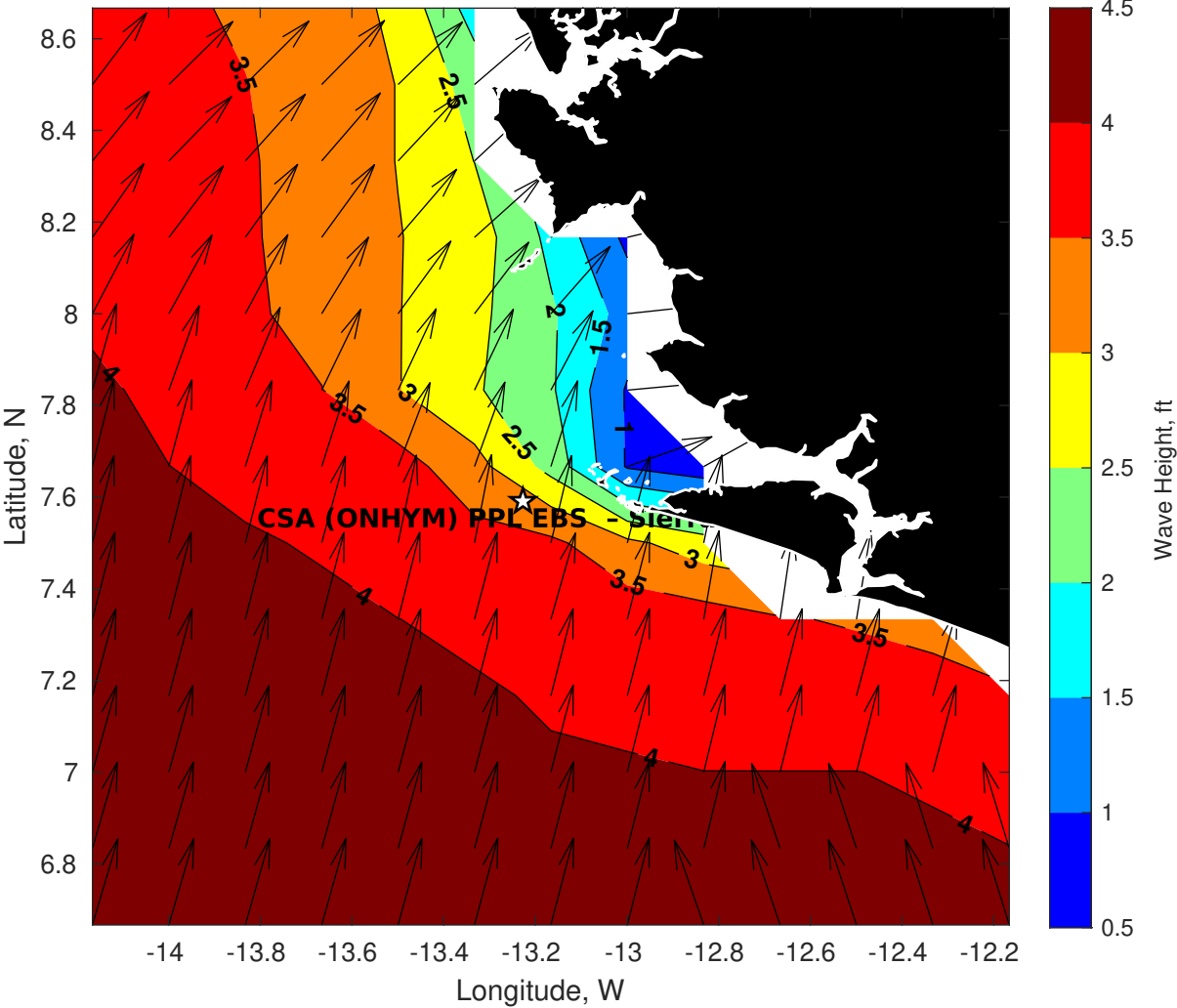
Wave Height (ft) for CSA (ONHYM) PPL EBS - Sierra Leone at 12-Jul-2025 09:00:00
