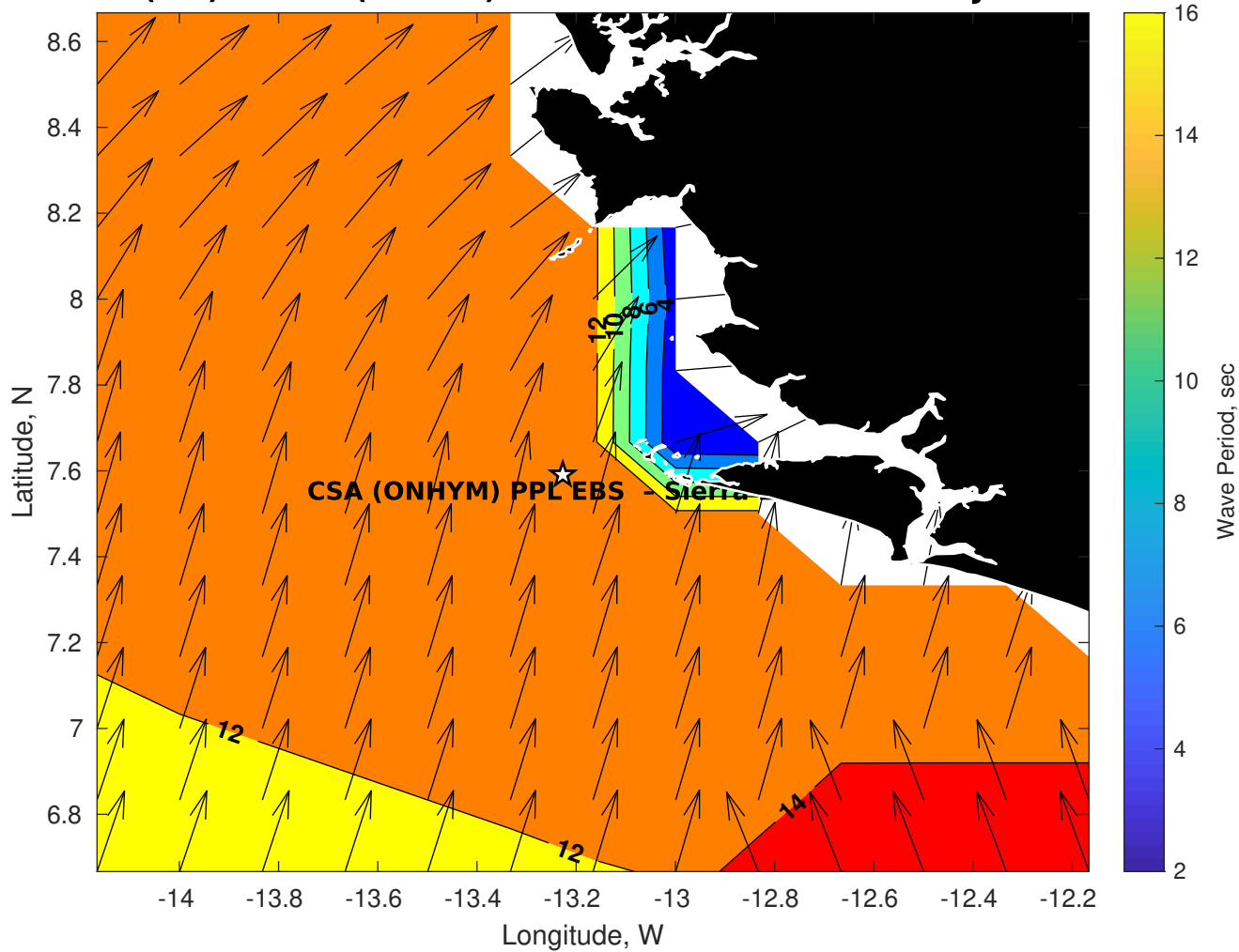
Wave Period (sec) for CSA (ONHYM) PPL EBS - Sierra Leone at 12-Jul-2025 09:00:00
