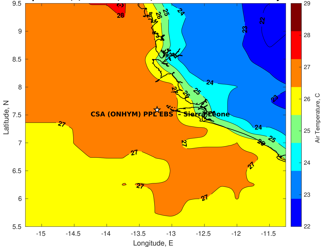
Air Temperature (C) for CSA (ONHYM) PPL EBS - Sierra Leone at 12-Jul-2025
