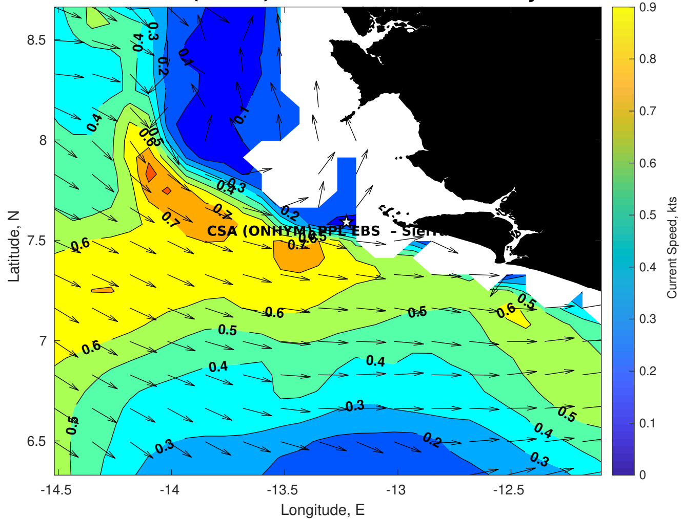
Surface Currents for CSA (ONHYM) PPL EBS - Sierra Leone at 11-Jul-2025 00:00:00
