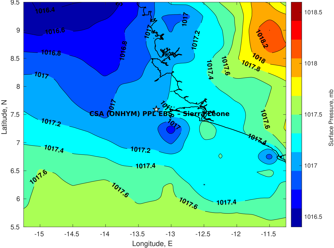
Surface Pressure (mb) for CSA (ONHYM) PPL EBS - Sierra Leone at 14-Jul-2025 00:00:00
