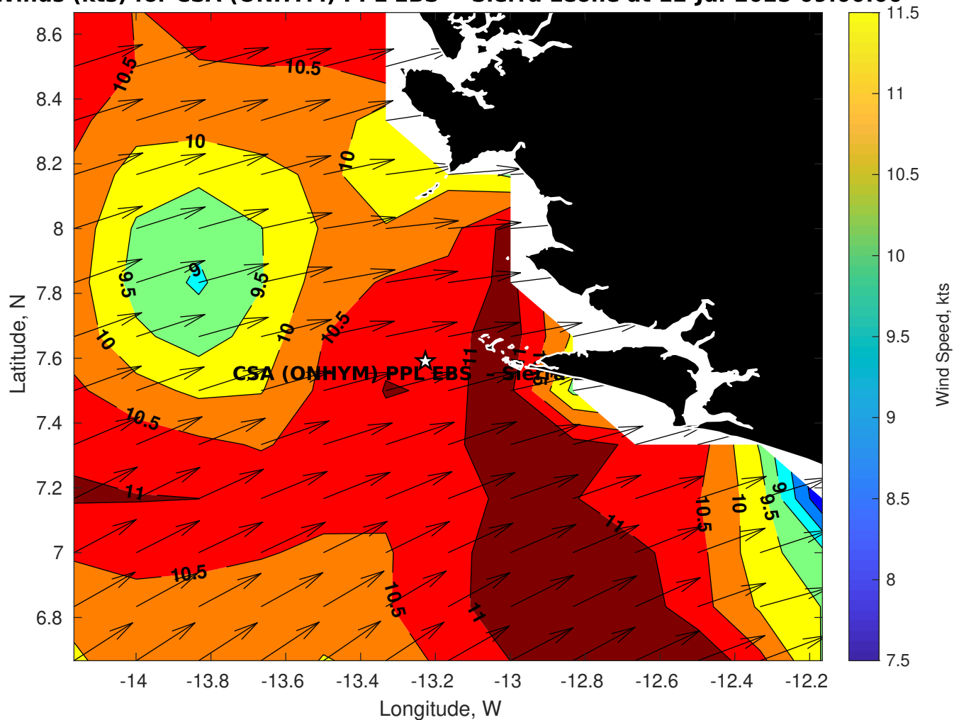
Winds (kts) for CSA (ONHYM) PPL EBS - Sierra Leone at 12-Jul-2025 09:00:00
