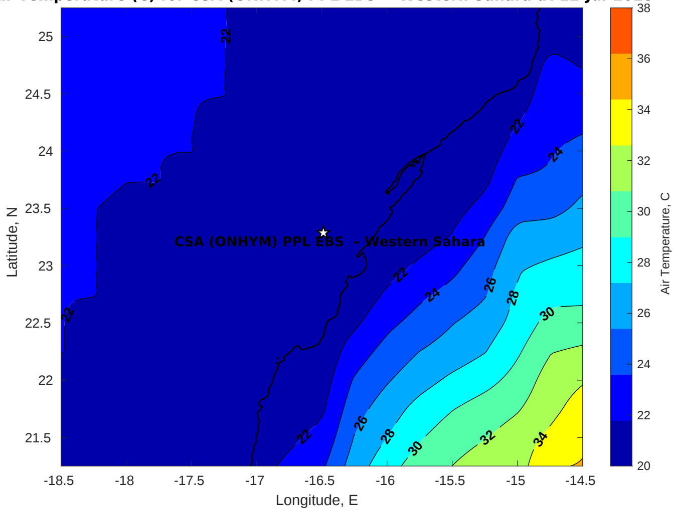
Air Temperature (C) for CSA (ONHYM) PPL EBS - Western Sahara at 12-Jul-2025
