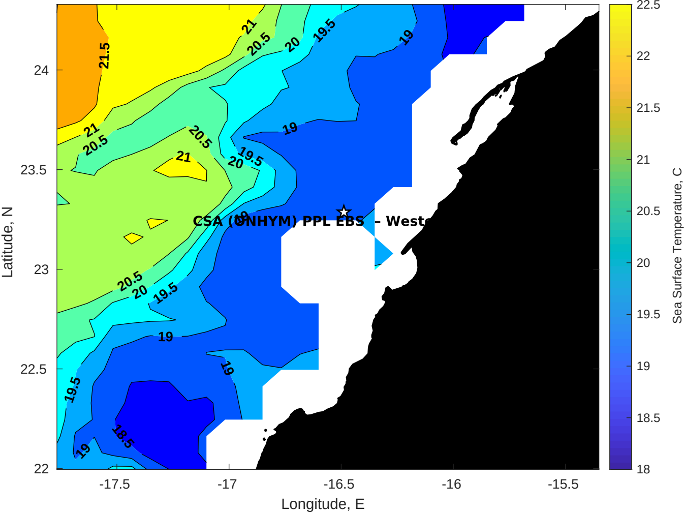
SST for CSA (ONHYM) PPL EBS - Western Sahara at 11-Jul-2025 00:00:00
