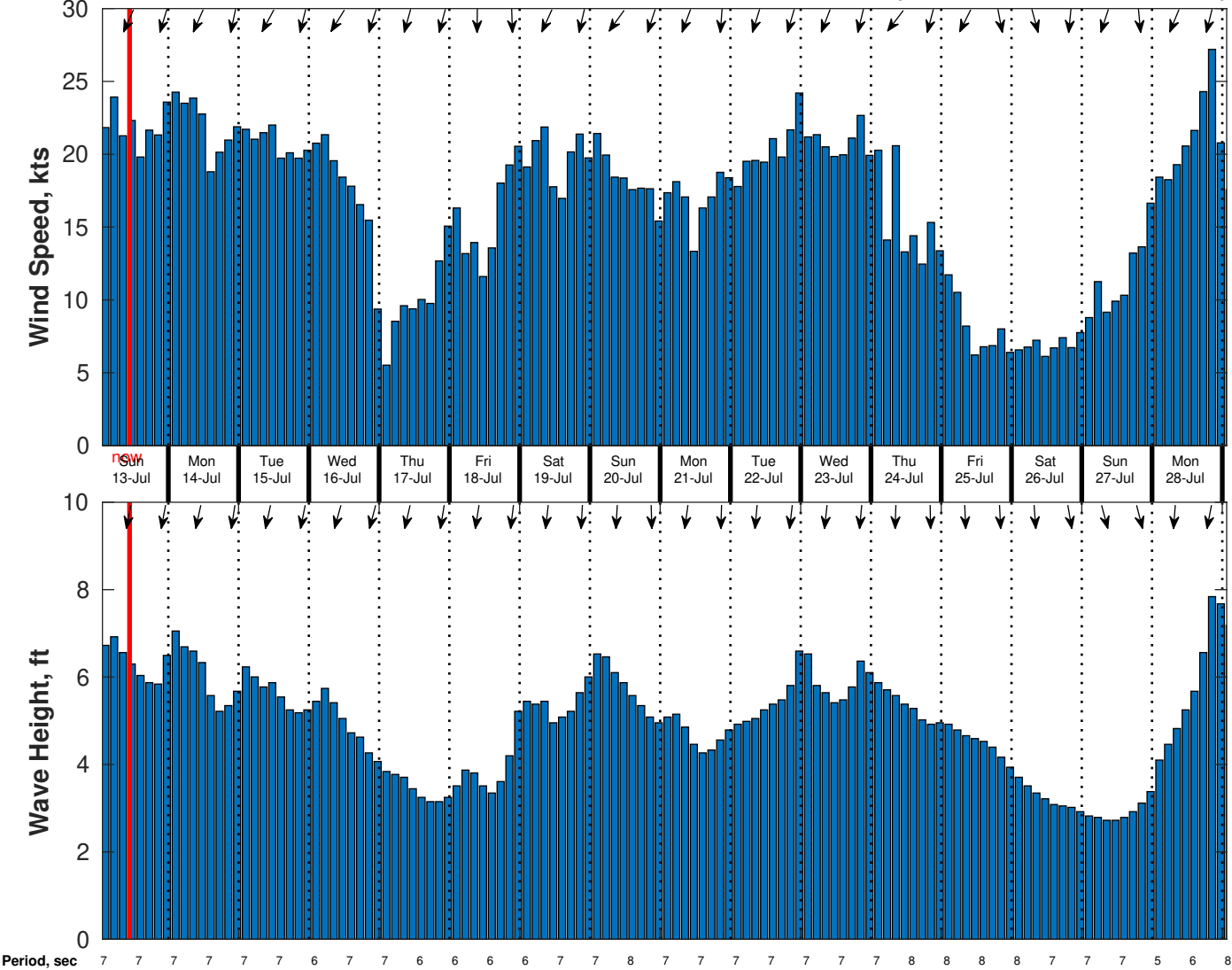
Wind & Wave Forecast for CSA (ONHYM) PPL EBS - Western Sahara from 12-Jul-2025 01:00:00 to 28-Jul-2025 01:00:00
