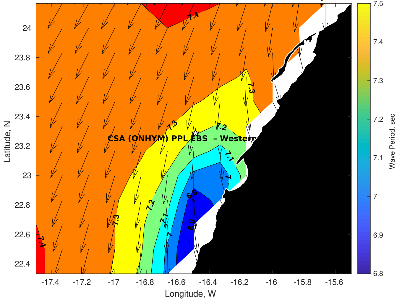
Wave Period (sec) for CSA (ONHYM) PPL EBS - Western Sahara at 12-Jul-2025 09:00:00
