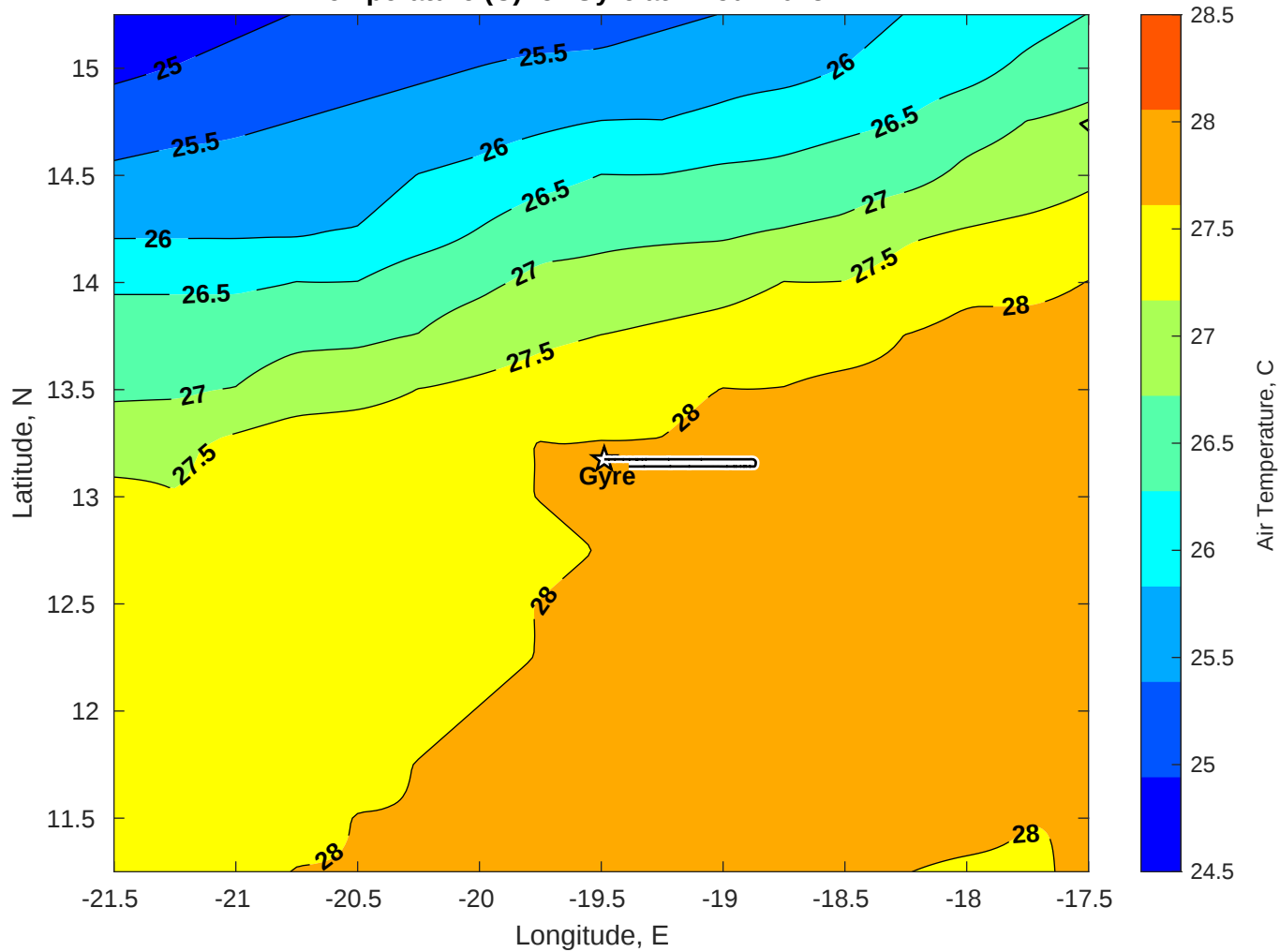
Air Temperature (C) for Gyre at 12-Jul-2025
