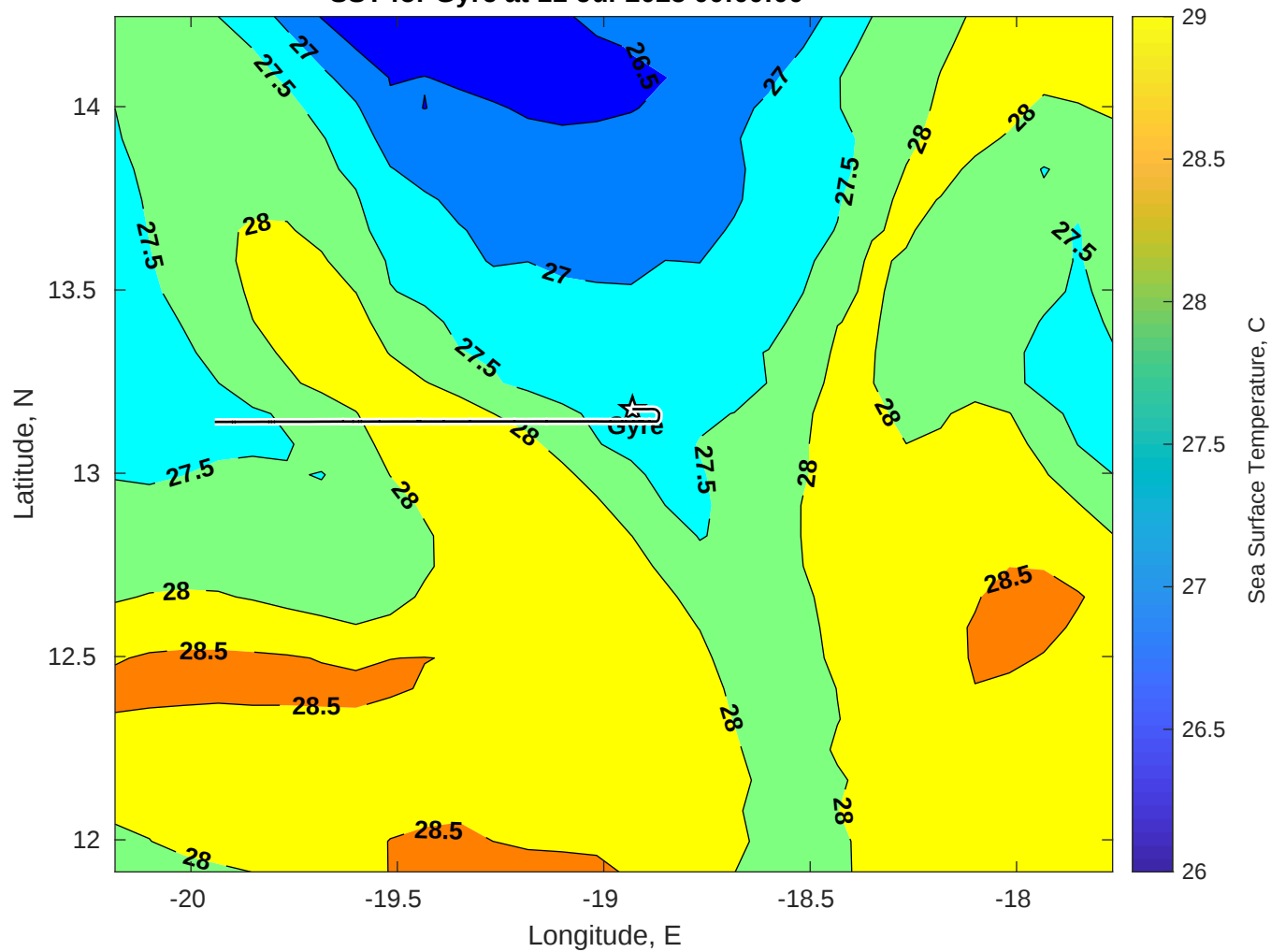
SST for Gyre at 11-Jul-2025 00:00:00
