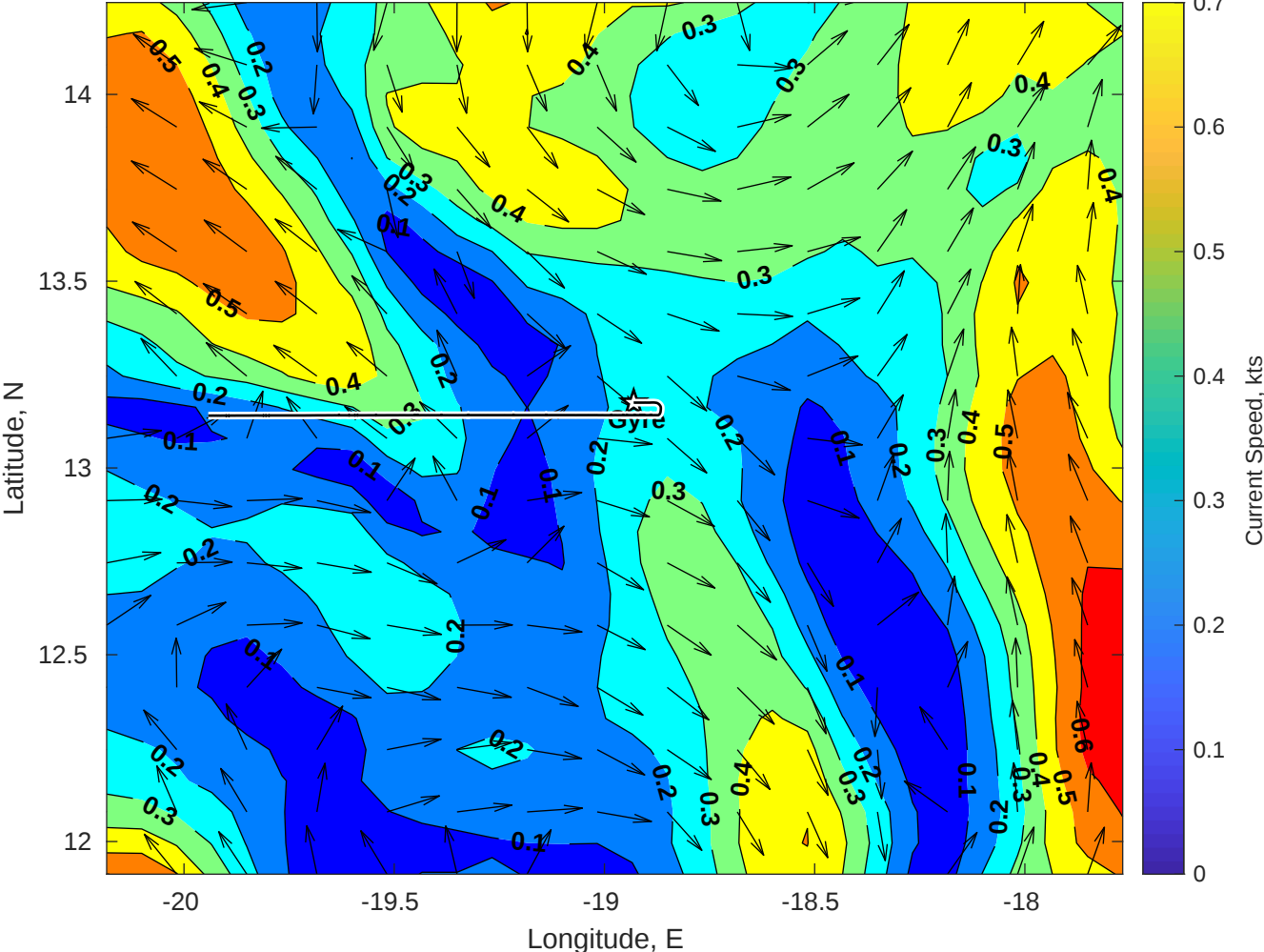
Surface Currents for Gyre at 11-Jul-2025 00:00:00
