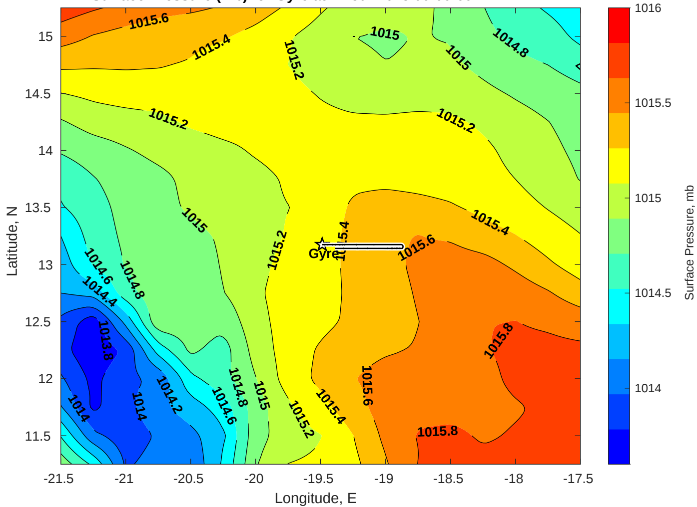
Surface Pressure (mb) for Gyre at 12-Jul-2025 00:00:00
