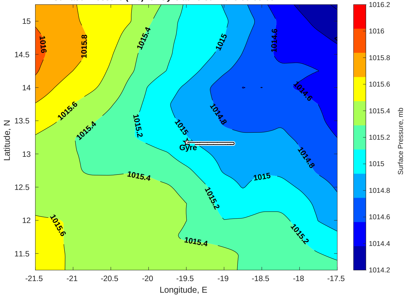
Surface Pressure (mb) for Gyre at 13-Jul-2025 00:00:00
