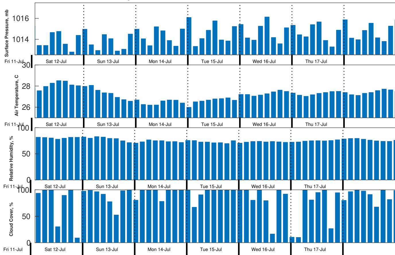
Met Forecast for Gyre from 11-Jul-2025 23:00:00 to 18-Jul-2025 23:00:00
