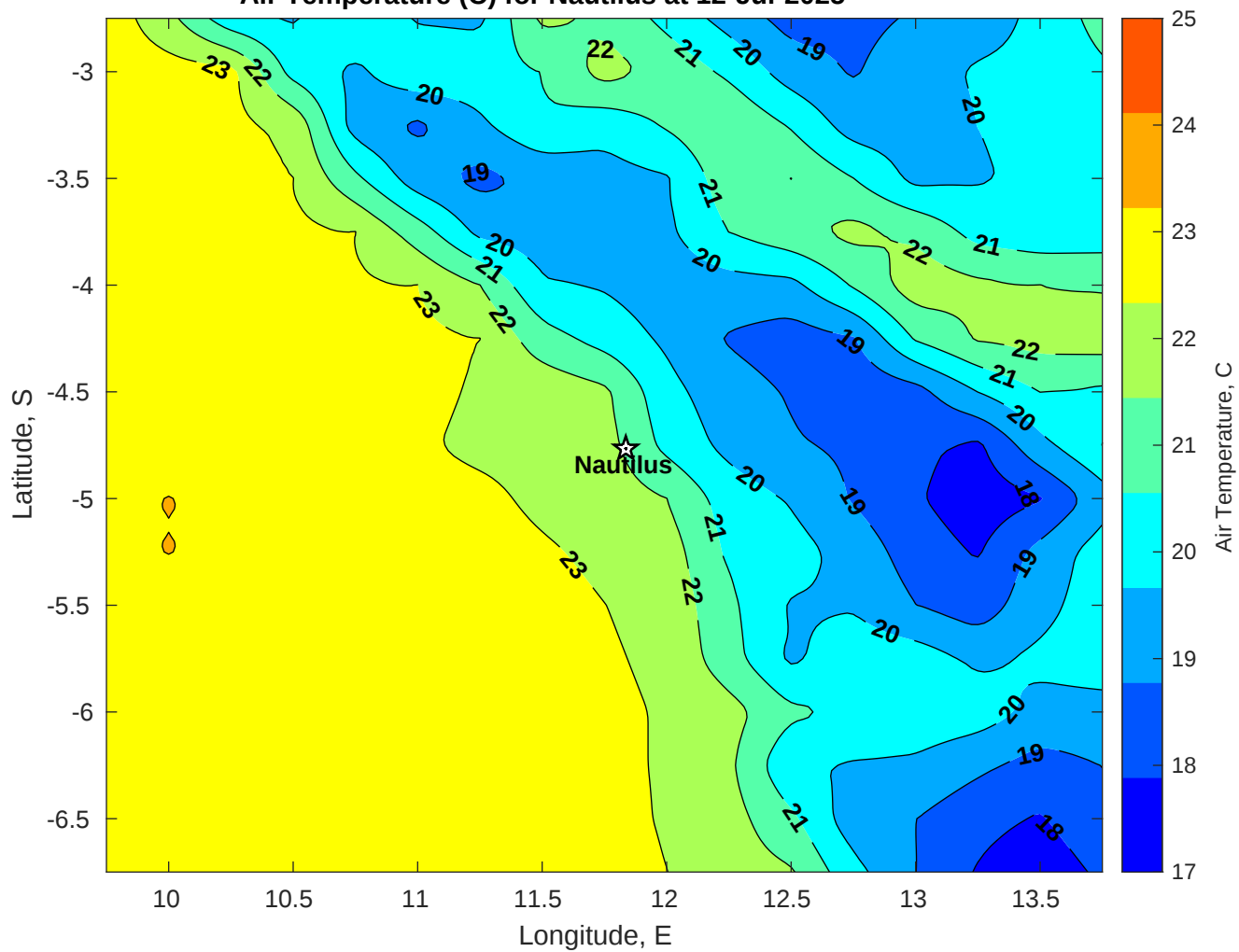
Air Temperature (C) for Nautilus at 12-Jul-2025
