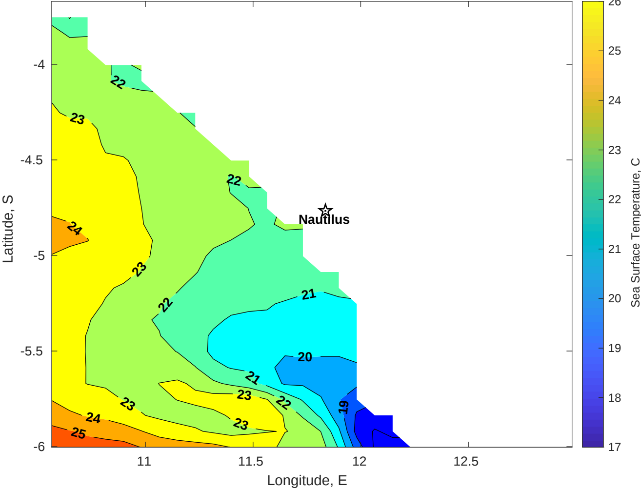
SST for Nautilus at 11-Jul-2025 00:00:00
