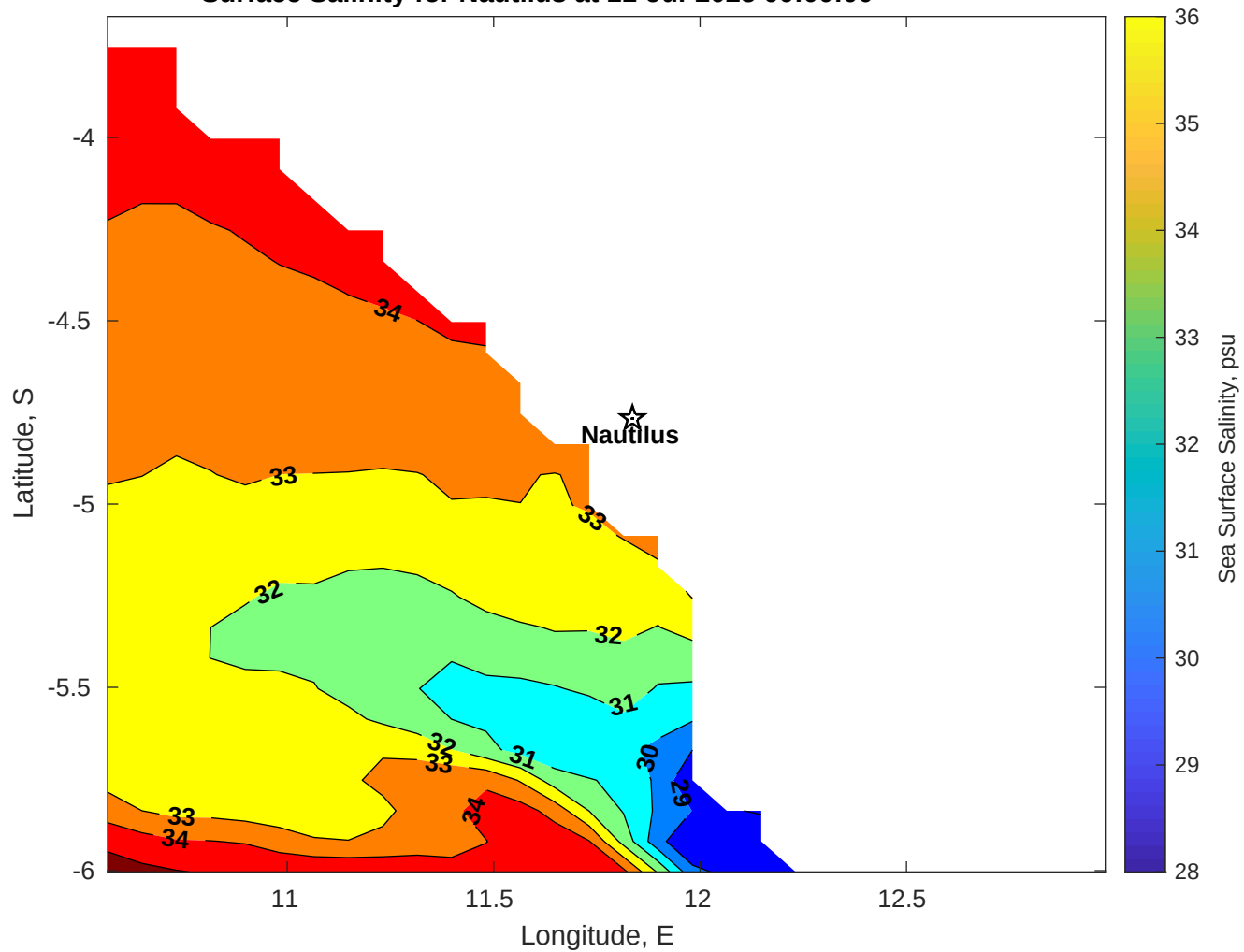
Surface Salinity for Nautilus at 11-Jul-2025 00:00:00
