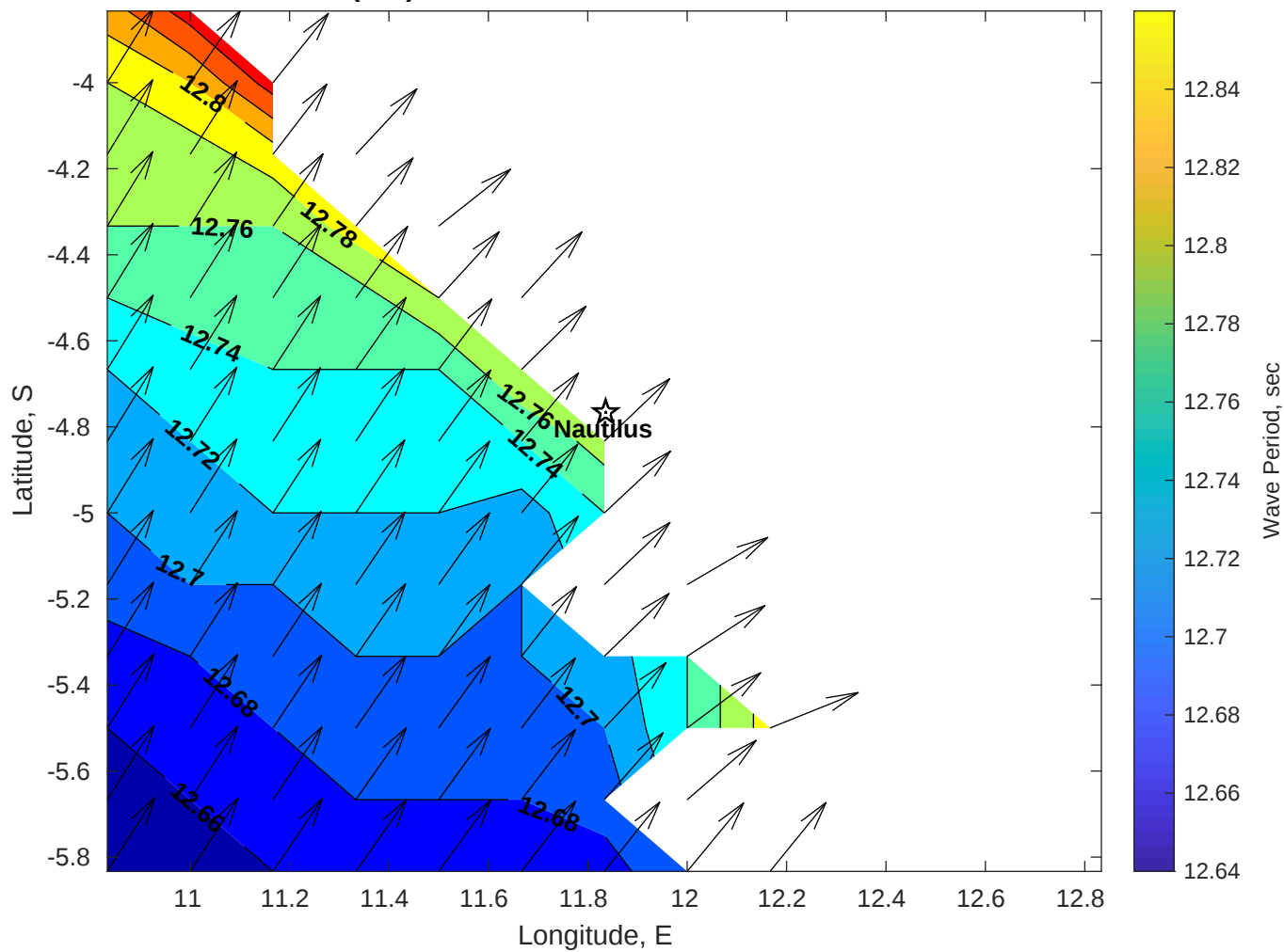
Wave Period (sec) for Nautilus at 12-Jul-2025 09:00:00
