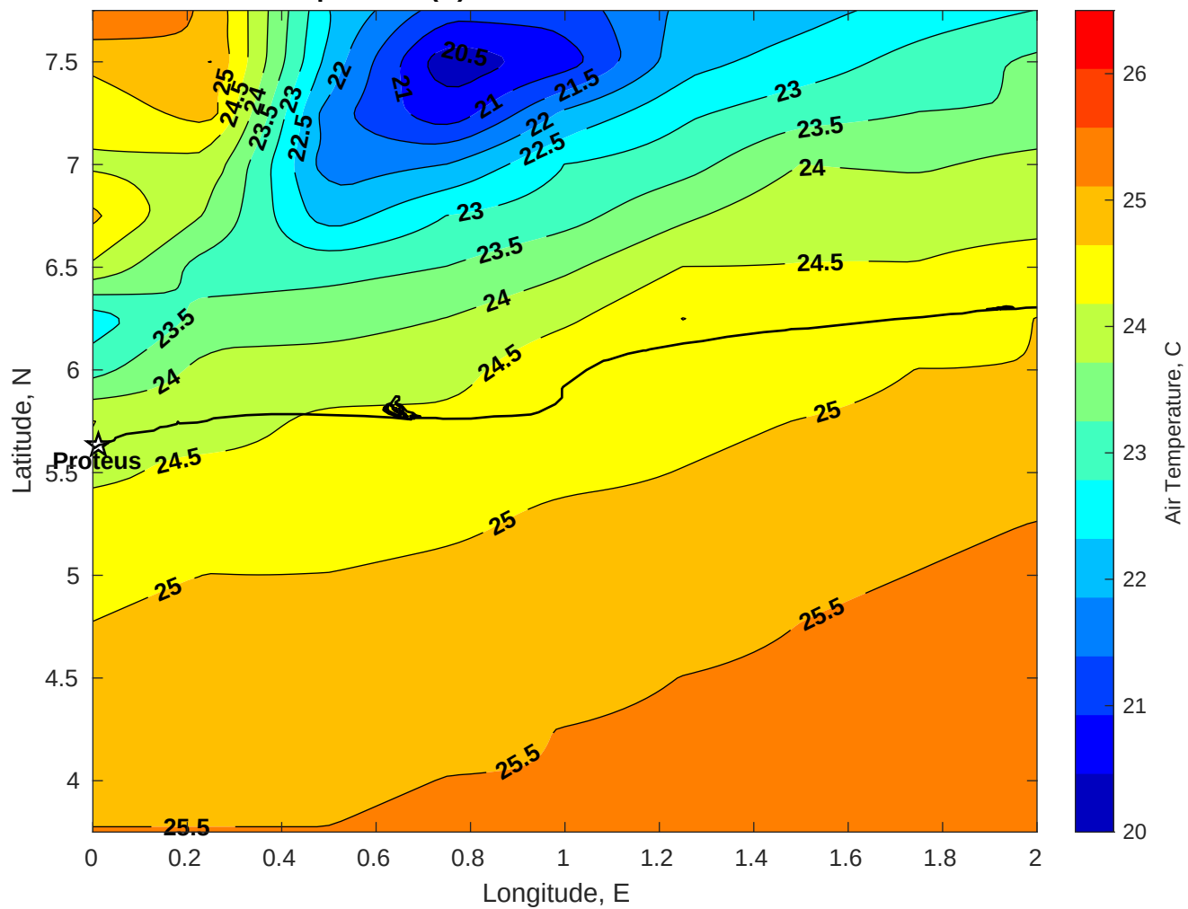
Air Temperature (C) for Proteus at 12-Jul-2025
