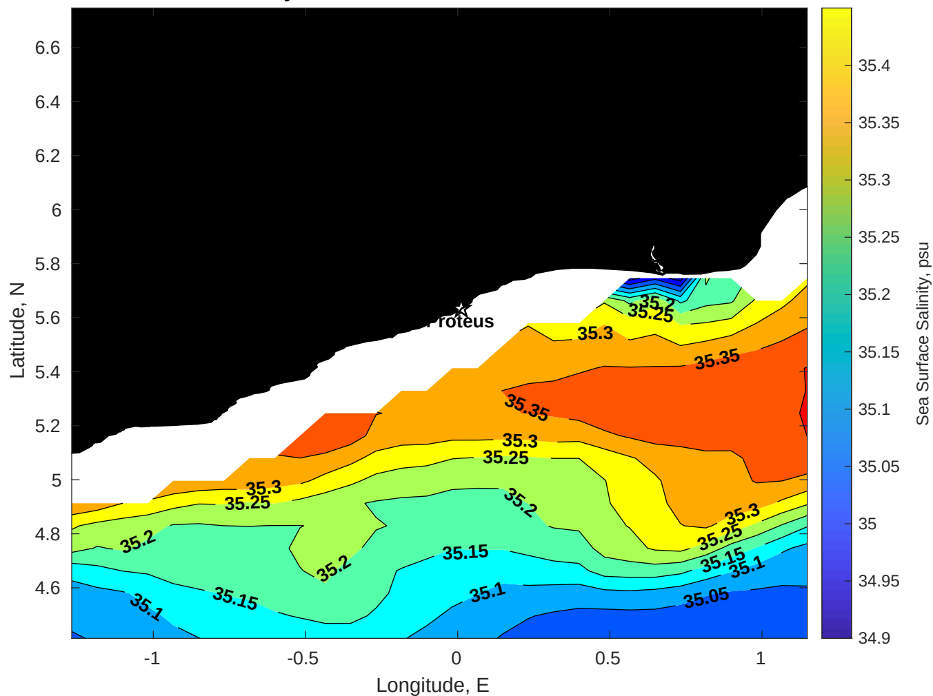
Surface Salinity for Proteus at 11-Jul-2025 00:00:00
