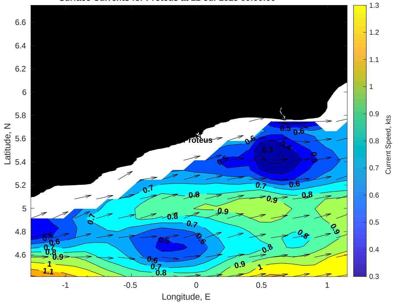
Surface Currents for Proteus at 11-Jul-2025 00:00:00
