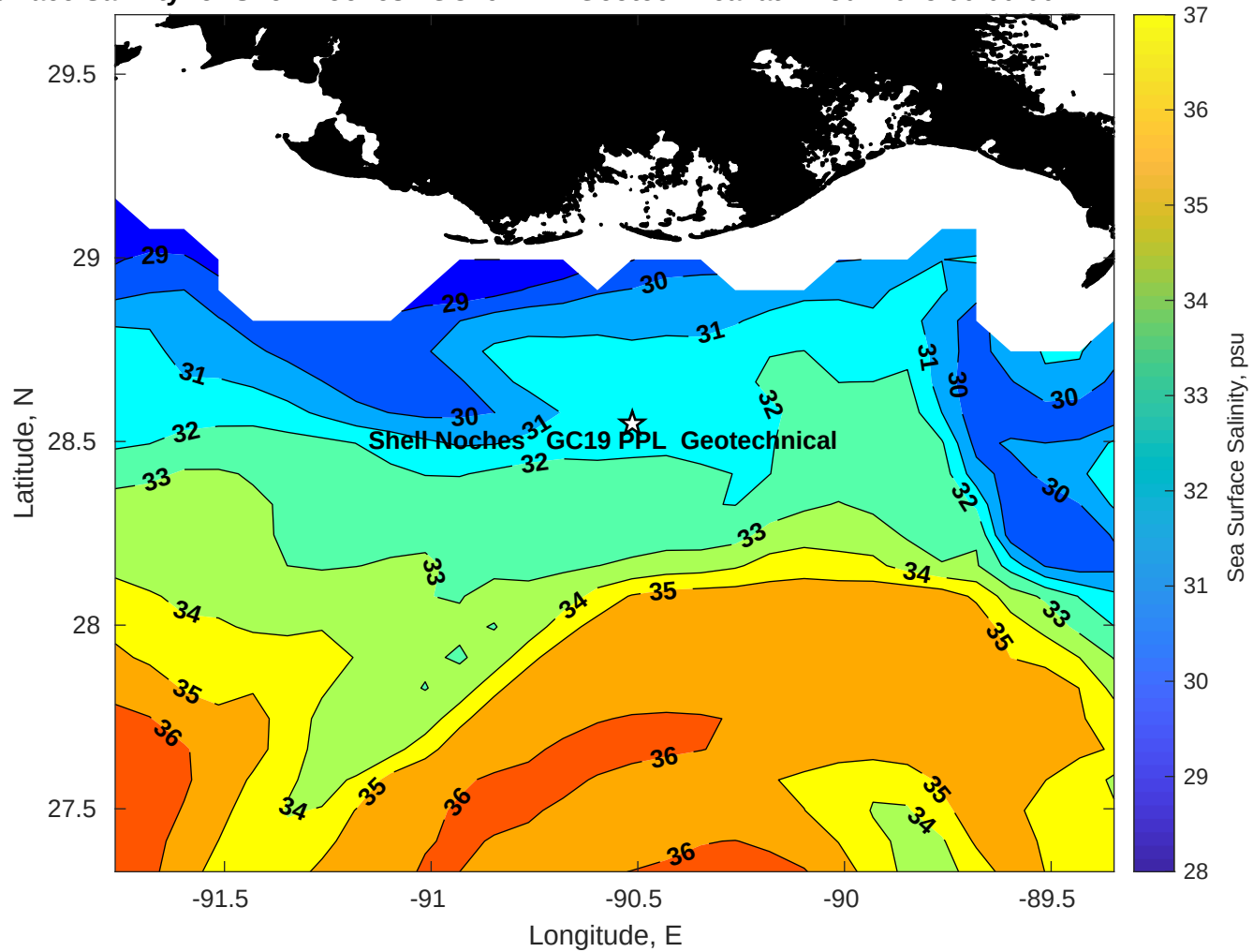
Surface Salinity for Shell Noches GC19 PPL Geotechnical at 11-Jul-2025 00:00:00
