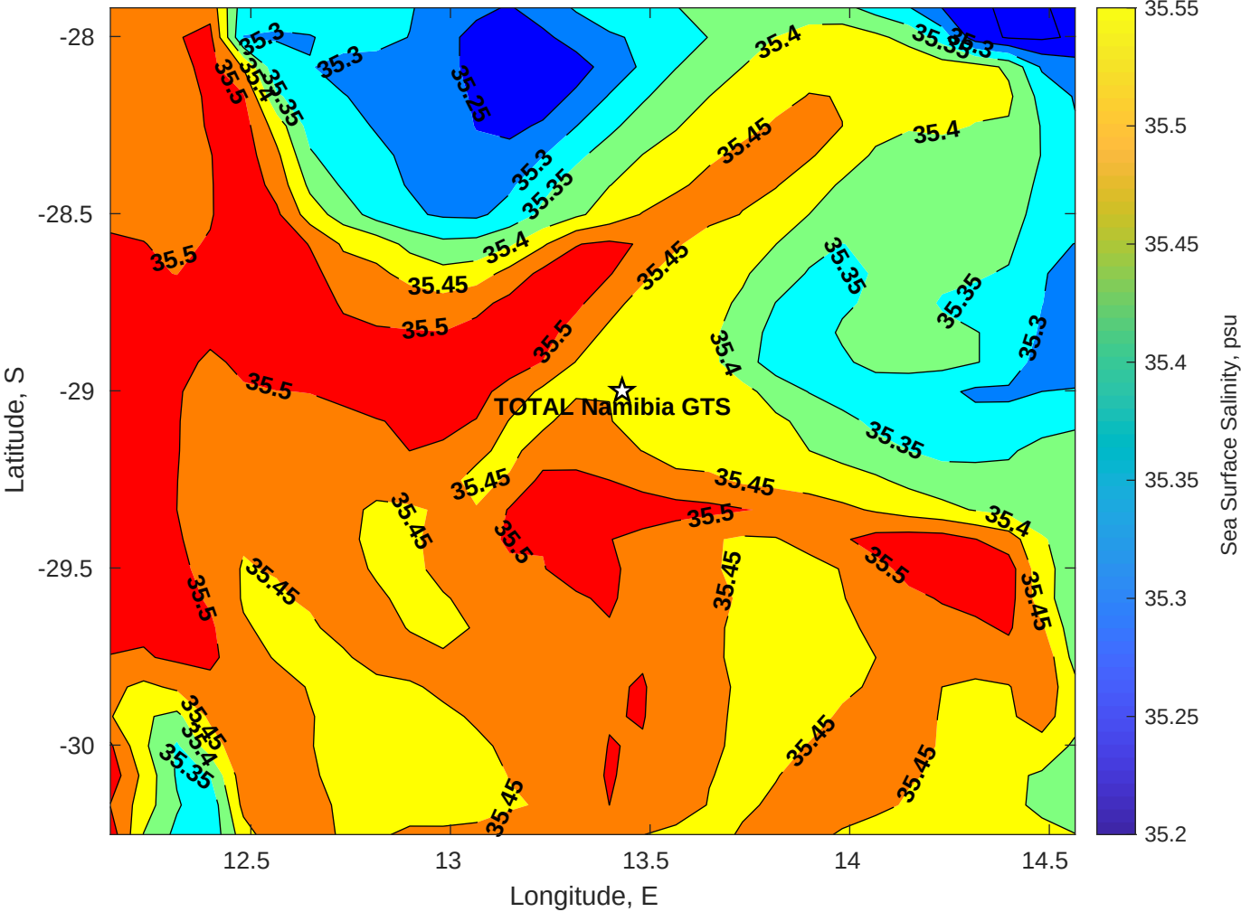
Surface Salinity for TOTAL Namibia GTS at 11-Jul-2025 00:00:00
