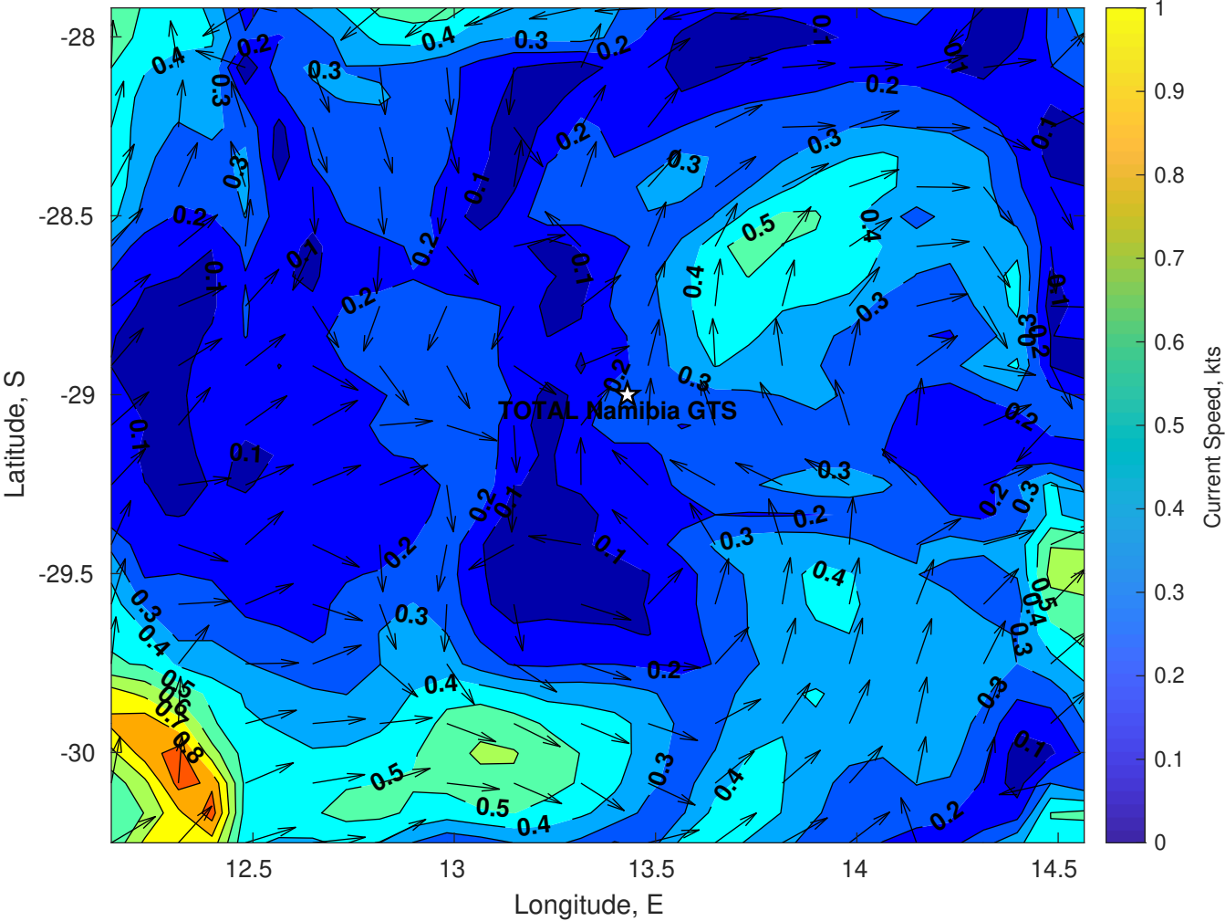
Surface Currents for TOTAL Namibia GTS at 11-Jul-2025 00:00:00
