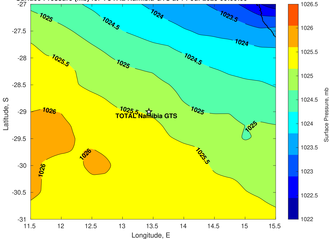
Surface Pressure (mb) for TOTAL Namibia GTS at 14-Jul-2025 00:00:00
