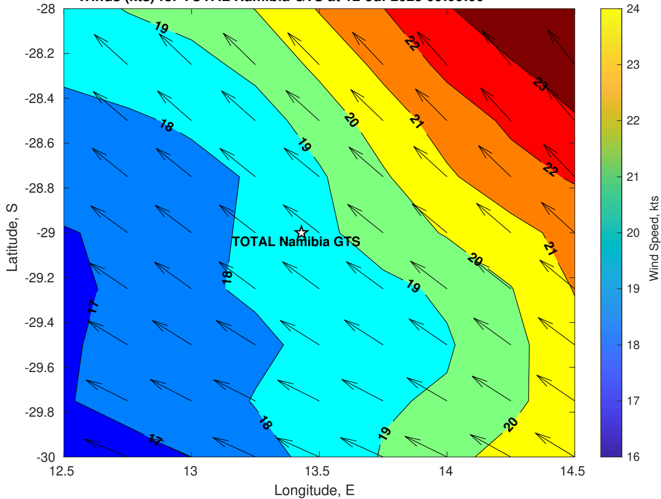
Winds (kts) for TOTAL Namibia GTS at 12-Jul-2025 09:00:00
