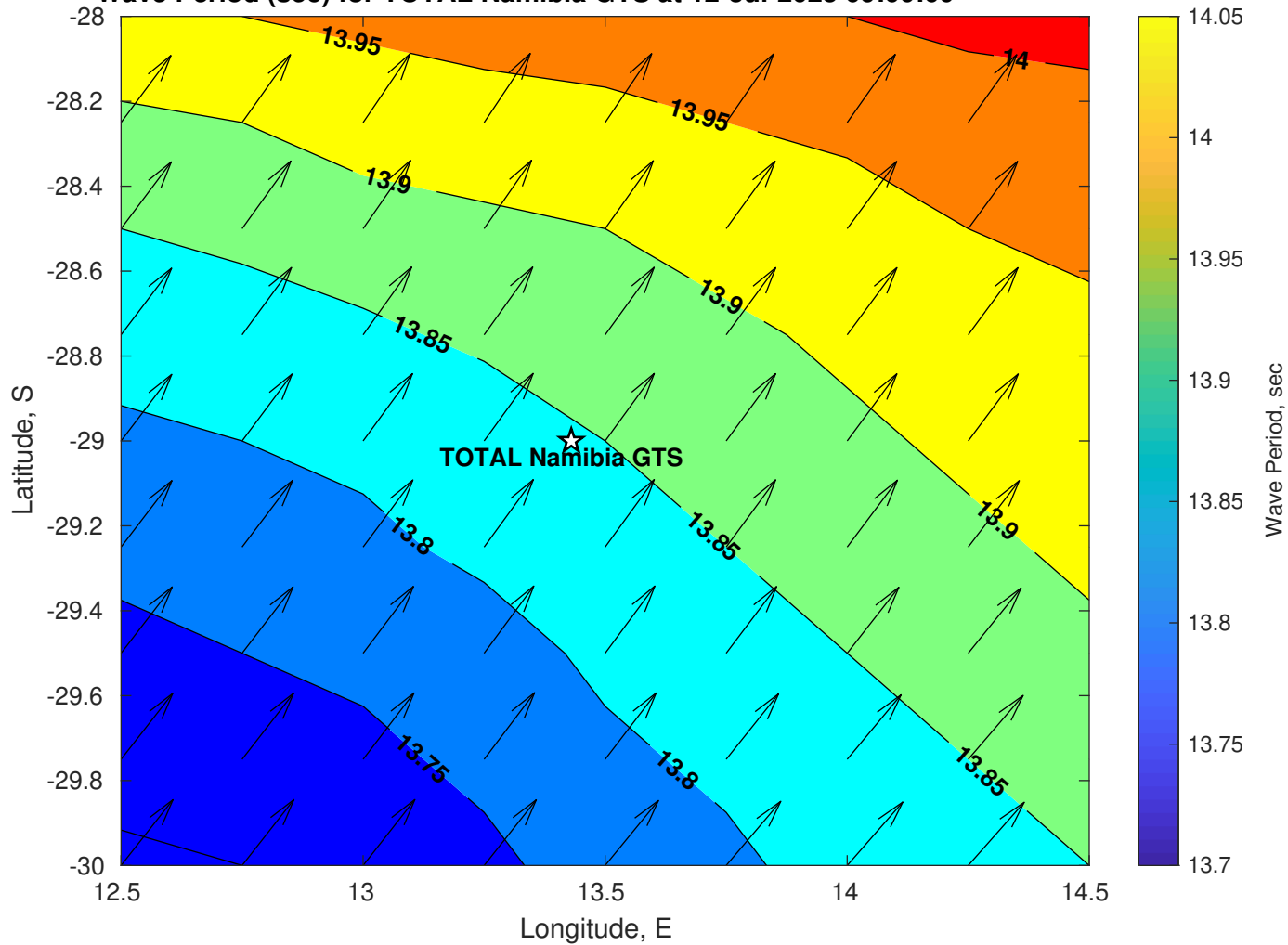
Wave Period (sec) for TOTAL Namibia GTS at 12-Jul-2025 09:00:00
