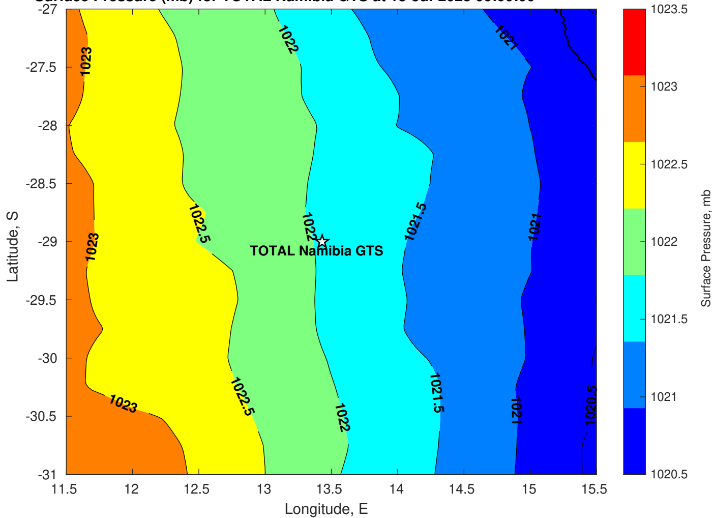
Surface Pressure (mb) for TOTAL Namibia GTS at 13-Jul-2025 00:00:00
