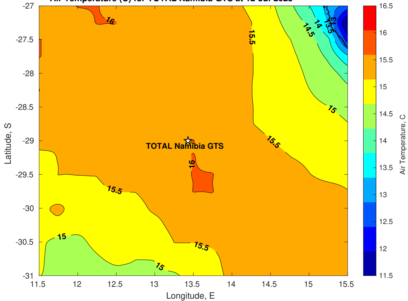
Air Temperature (C) for TOTAL Namibia GTS at 12-Jul-2025
