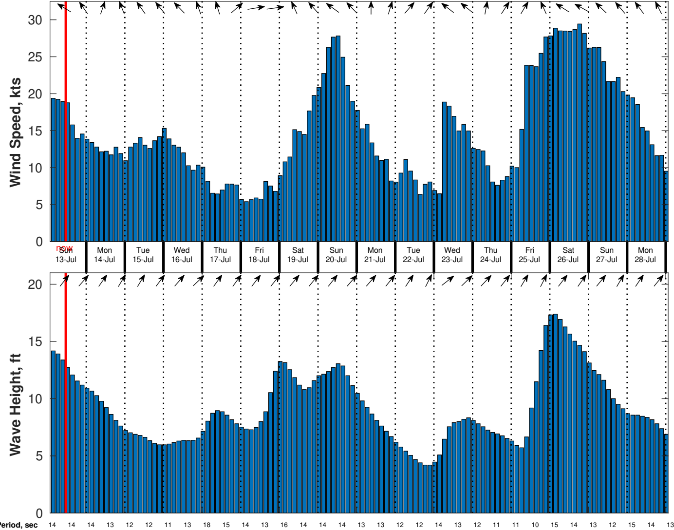
Wind & Wave Forecast for TOTAL Namibia GTS from 12-Jul-2025 02:00:00 to 28-Jul-2025 02:00:00
