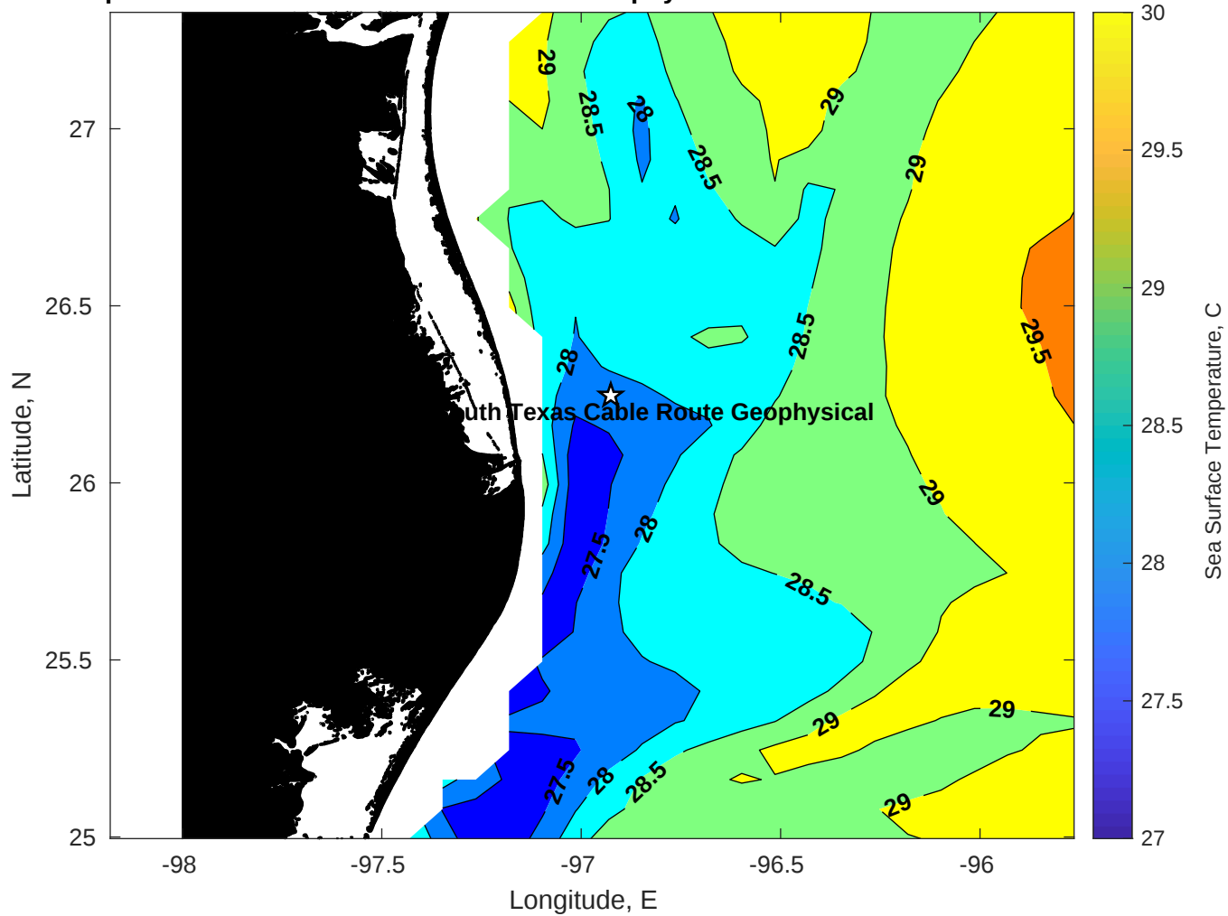
SST for Tampnet P2378 South Texas Cable Route Geophysical at 11-Jul-2025 00:00:00
