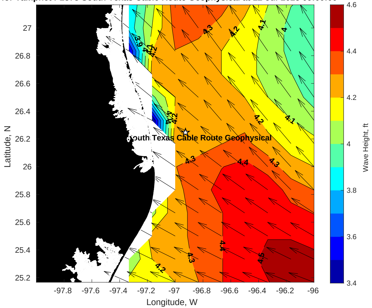
Wave Height (ft) for Tampnet P2378 South Texas Cable Route Geophysical at 12-Jul-2025 09:00:00
