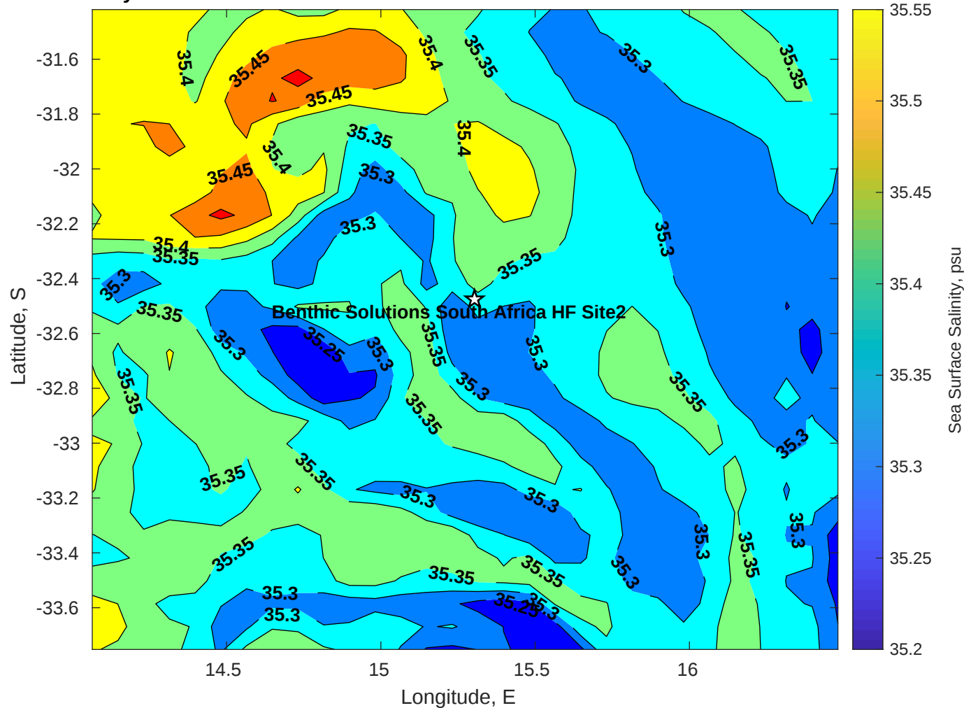
Surface Salinity for Benthic Solutions South Africa HF Site2 at 12-Jul-2025 00:00:00
