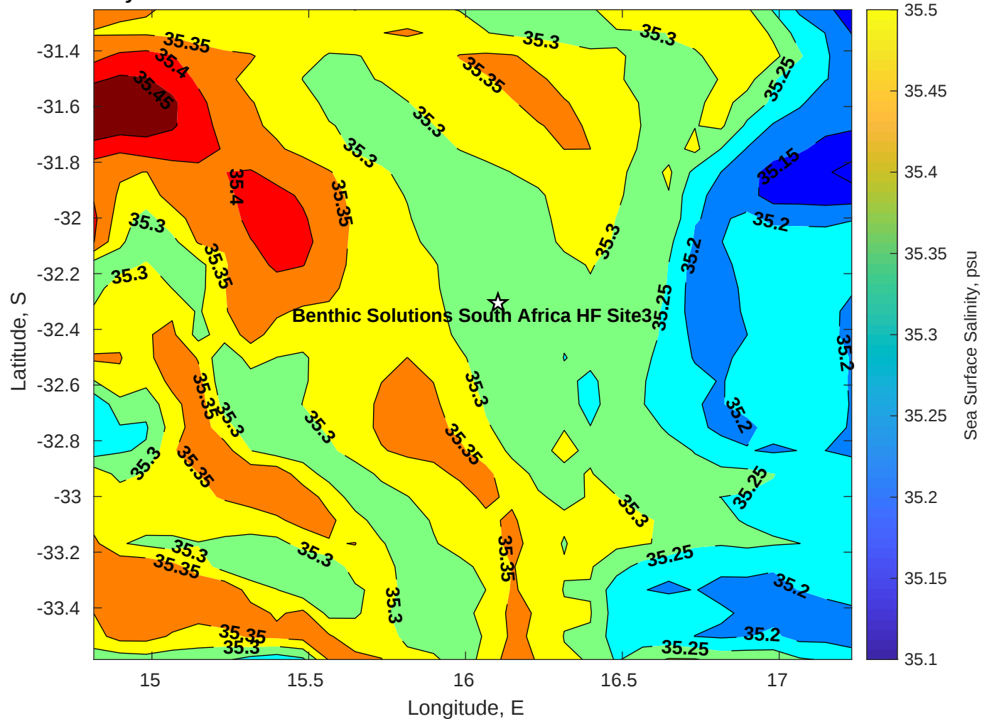
Surface Salinity for Benthic Solutions South Africa HF Site3 at 12-Jul-2025 00:00:00
