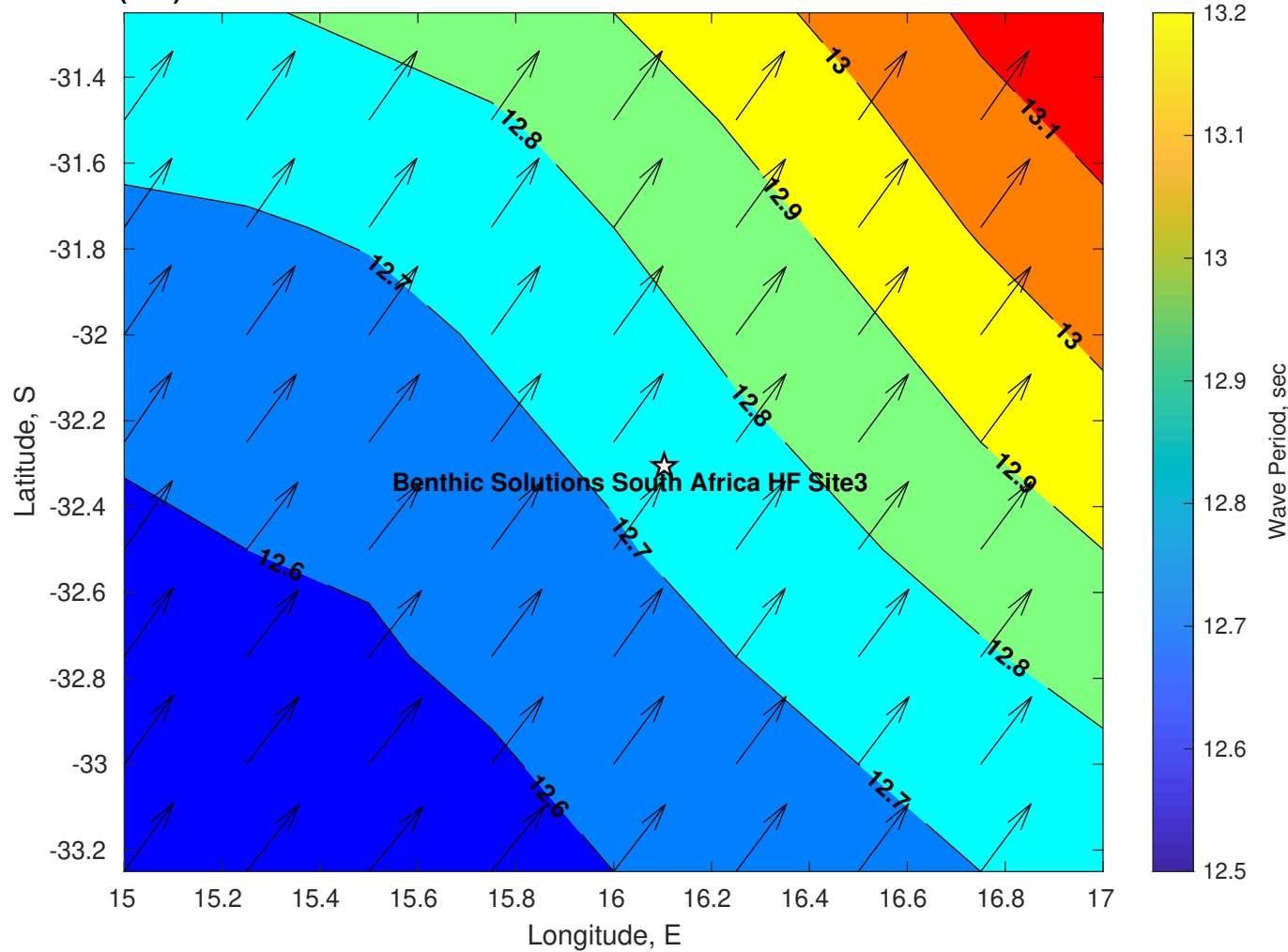
Wave Period (sec) for Benthic Solutions South Africa HF Site3 at 13-Jul-2025 09:00:00
