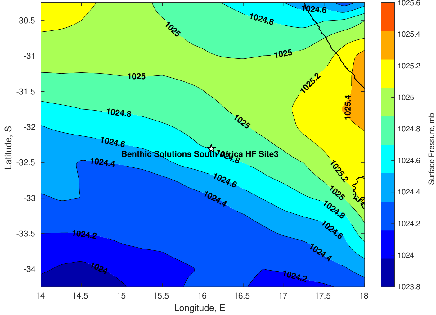
Surface Pressure (mb) for Benthic Solutions South Africa HF Site3 at 15-Jul-2025 00:00:00
