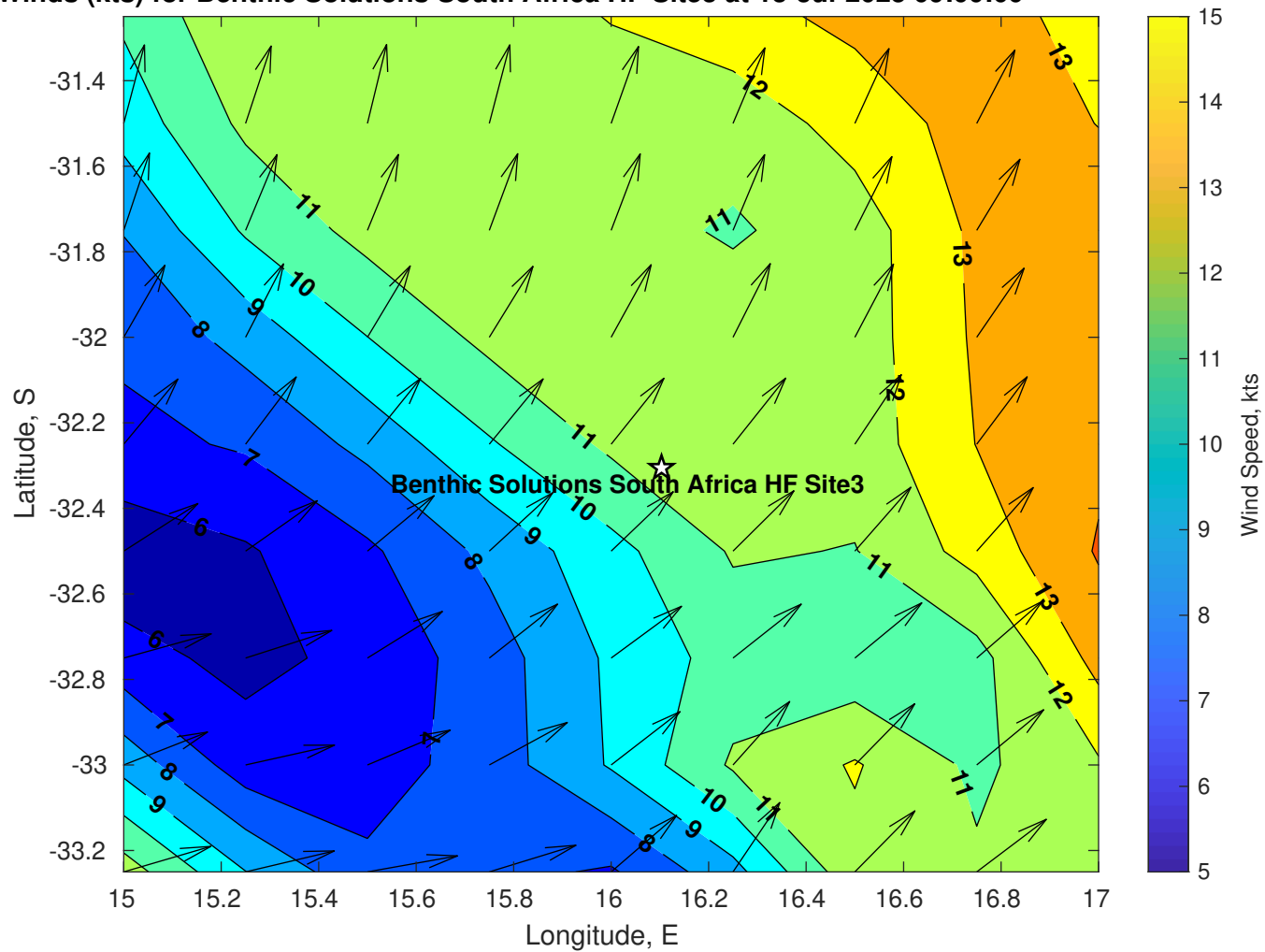
Winds (kts) for Benthic Solutions South Africa HF Site3 at 13-Jul-2025 09:00:00
