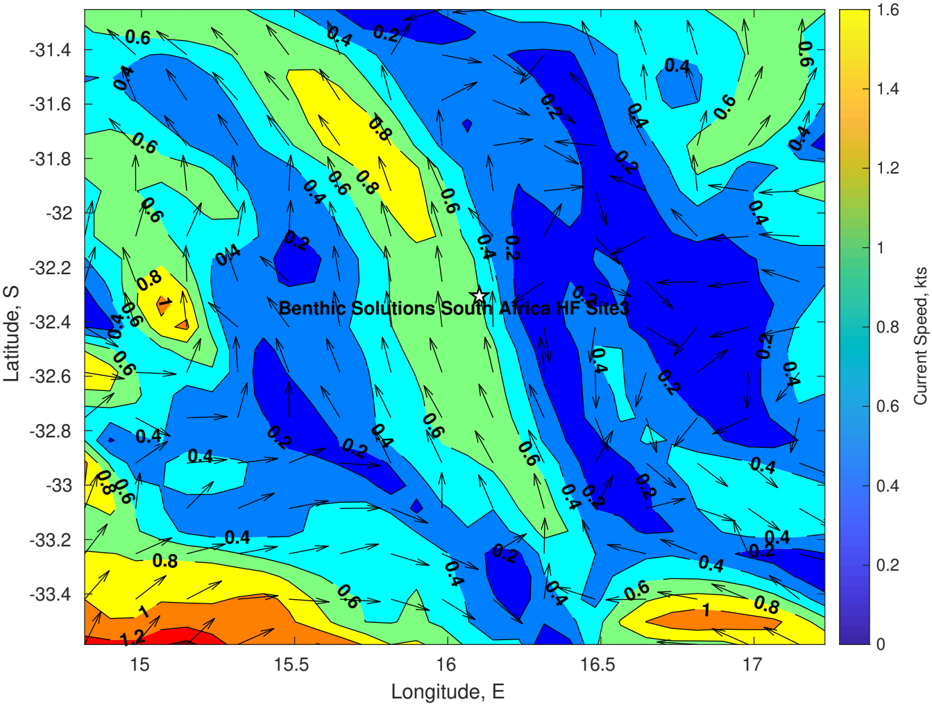
Surface Currents for Benthic Solutions South Africa HF Site3 at 12-Jul-2025 00:00:00
