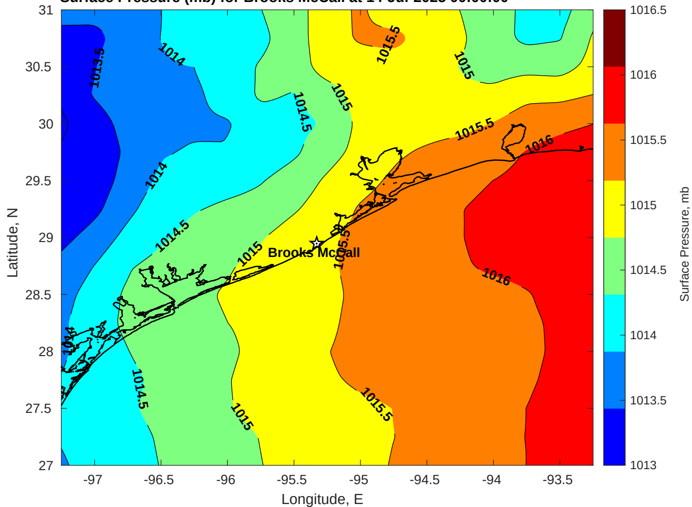
Surface Pressure (mb) for Brooks McCall at 14-Jul-2025 00:00:00
