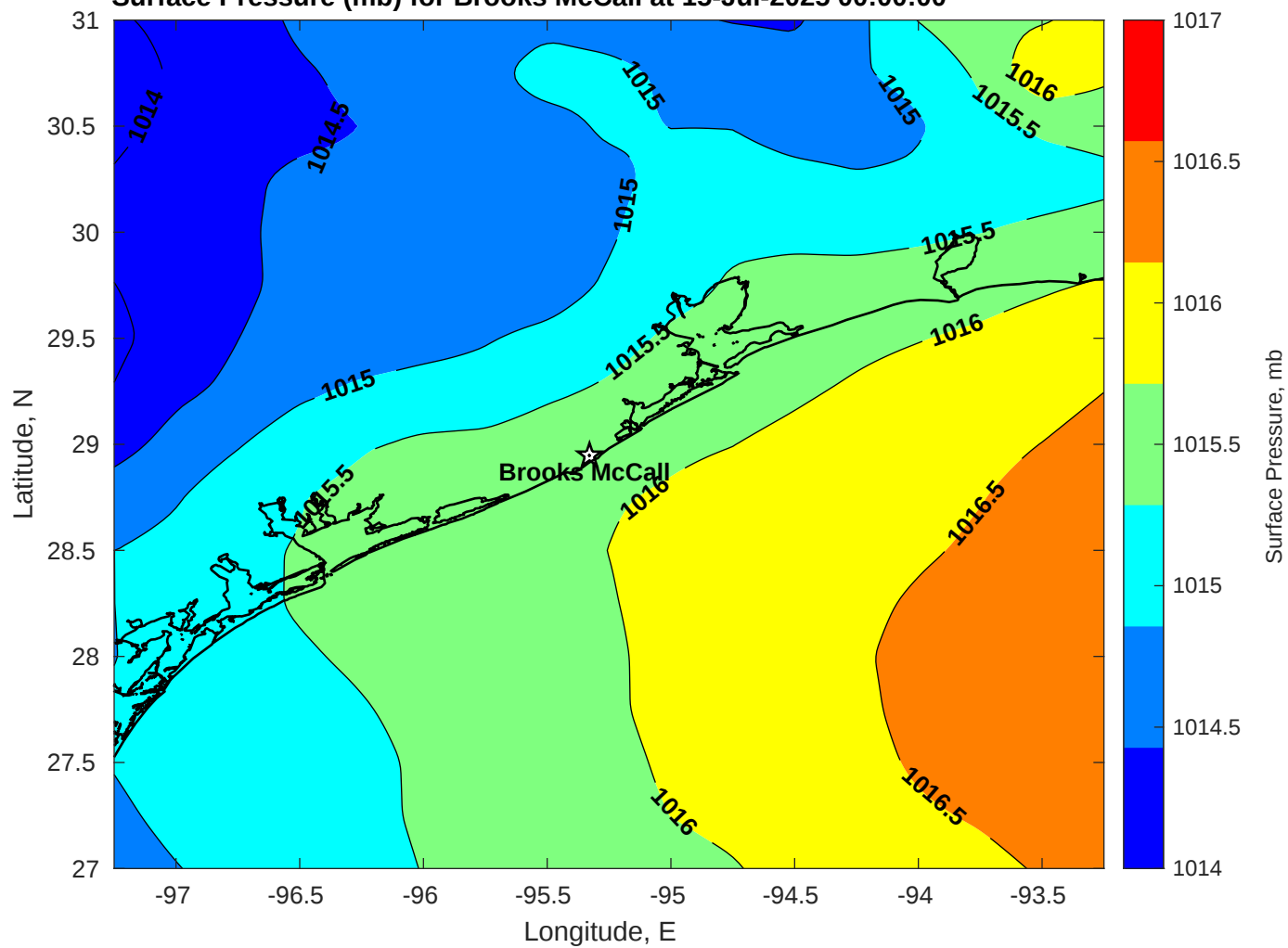
Surface Pressure (mb) for Brooks McCall at 15-Jul-2025 00:00:00
