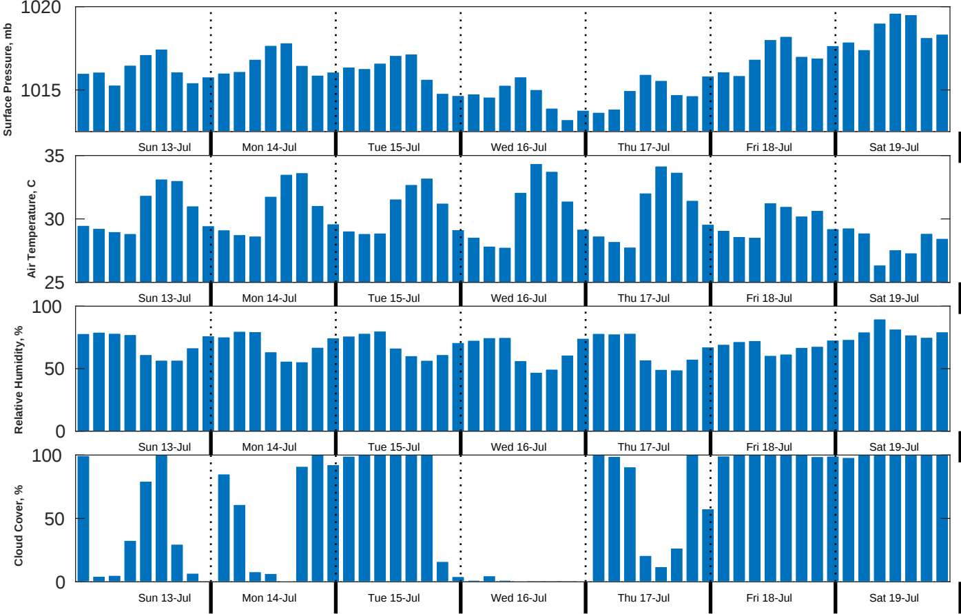
Met Forecast for Brooks McCall from 13-Jul-2025 00:00:00 to 20-Jul-2025 00:00:00
