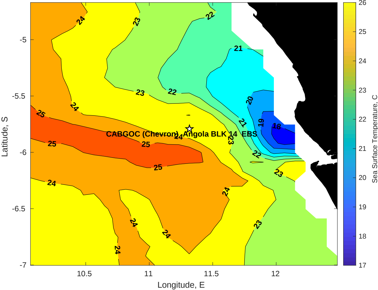
SST for CABGOC (Chevron) Angola BLK 14 EBS at 12-Jul-2025 00:00:00
